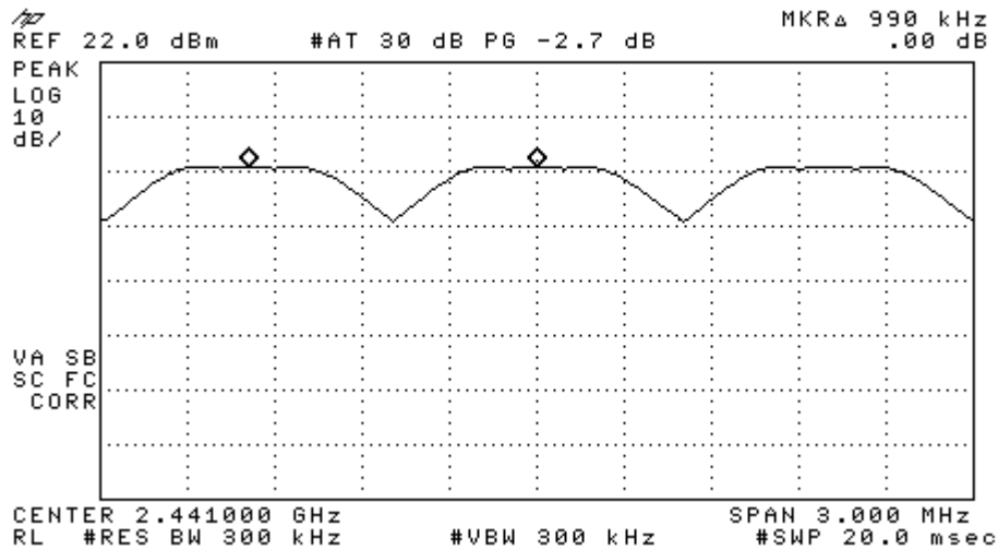
Figure 4: Carrier Frequency Separation between channels 38, 39 (mid-channel) & 40.
