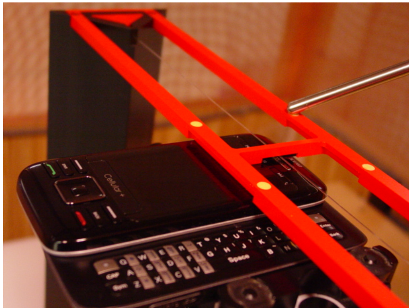
Figure 2b - HAC T-Coil Test Setup for Opened Configuration
