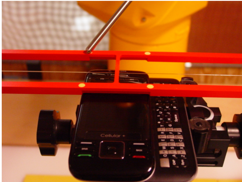
Figure 2a - HAC T-Coil Test Setup for Opened Configuration
