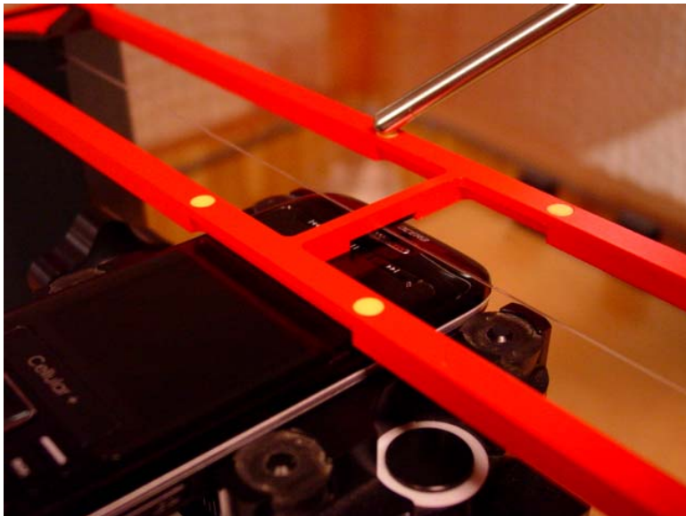
Figure 1b - HAC T-Coil Test Setup for Closed Configuration
