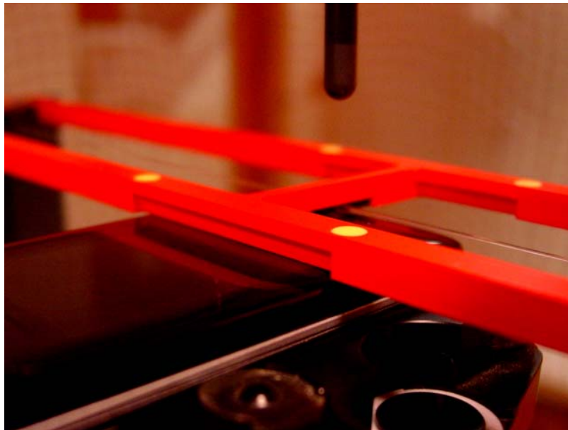
Figure 1b – HAC RF Emission Test Setup for Closed Configuration
