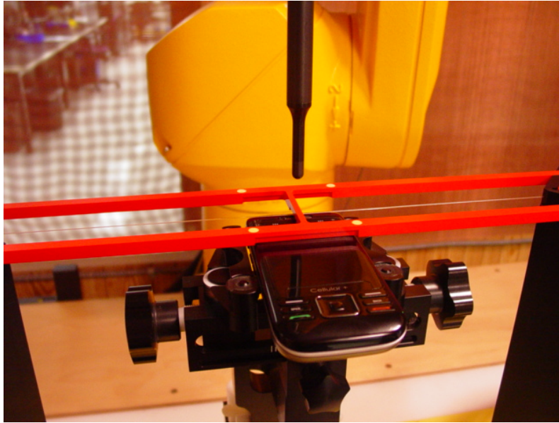
Figure 1a – HAC RF Emission Test Setup for Closed Configuration
