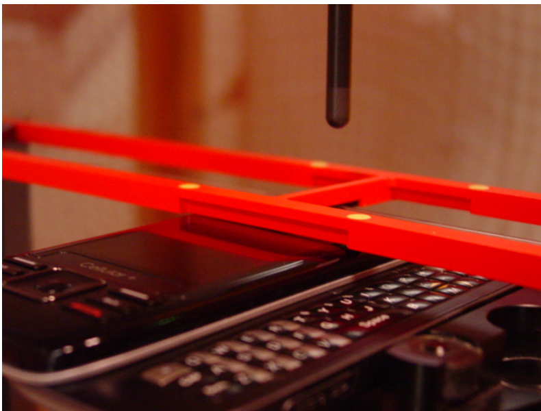
Figure 2b – HAC RF Emission Test Setup for Opened Configuration
