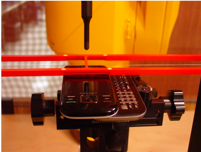
Figure 2a – HAC RF Emission Test Setup for Opened Configuration
