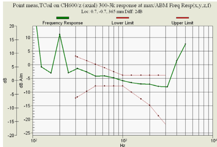
Figure 10.2b CDMA 1900 Channel 600 Closed Frequency Response
