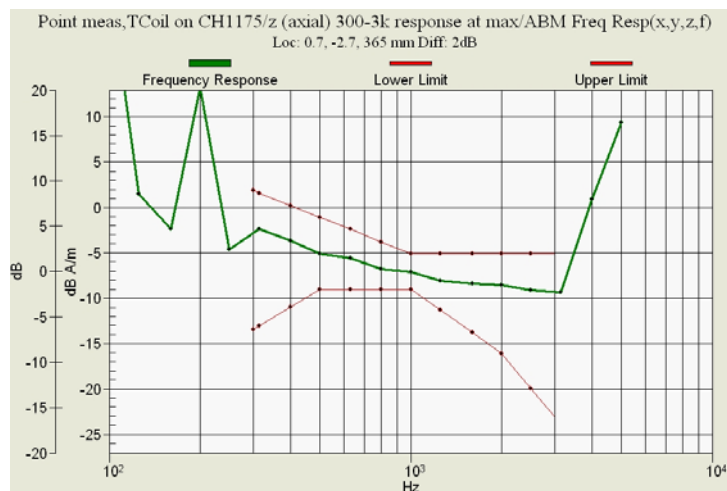
Figure 10.2c CDMA 1900 Channel 1175 Closed Frequency Response
