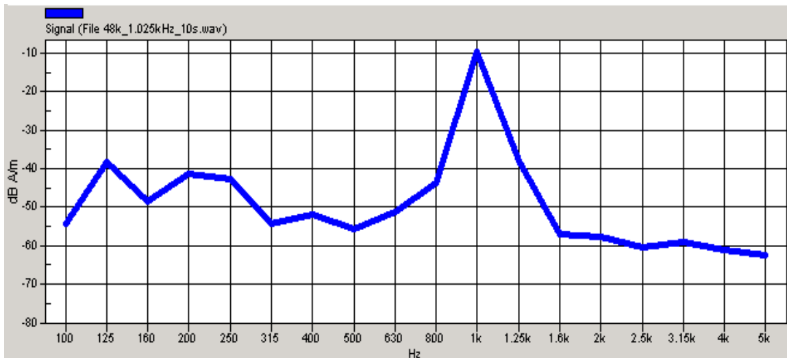
Figure 7.2a 1.025 KHz Voice signal spectrum
