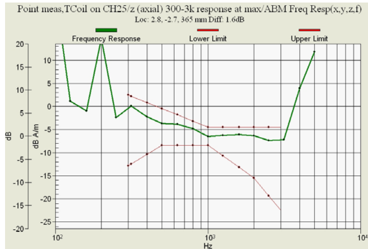
Figure 10.2d CDMA 1900 Channel 25 Opened Frequency Response
