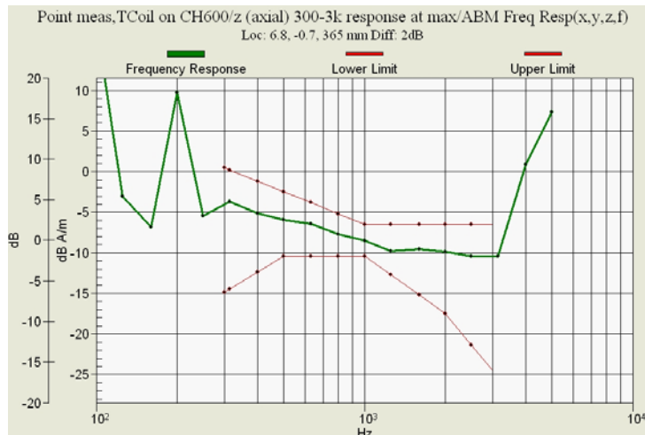
Figure 10.2e CDMA 1900 Channel 600 Opened Frequency Response
