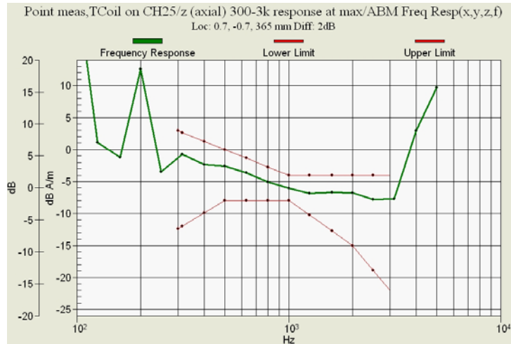
Figure 10.2a CDMA 1900 Channel 25 Closed Frequency Response
