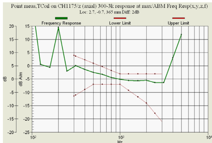
Figure 10.2f CDMA 1900 Channel 1175 Opened Frequency Response
