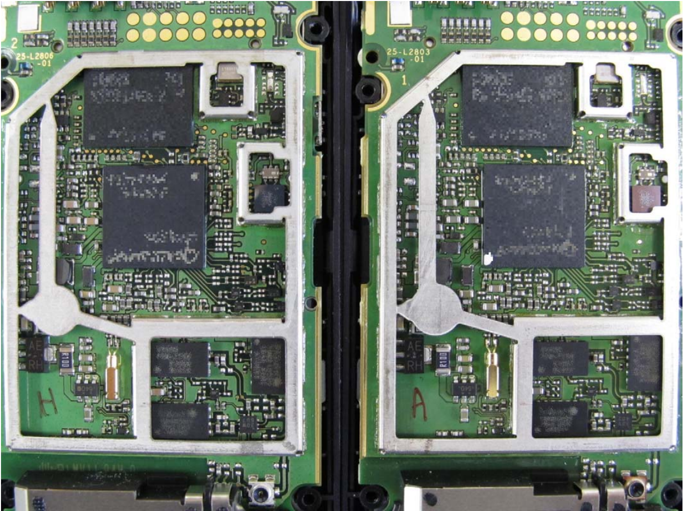
“B” PWB
