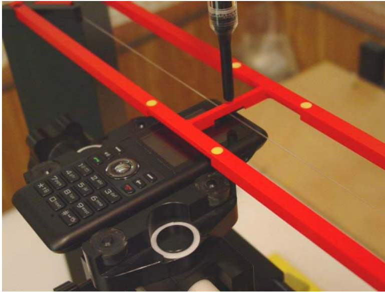
Figure 1a – HAC RF Setup Photo
