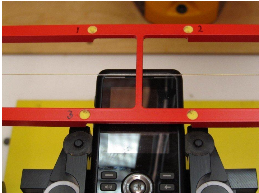
Figure 1b – HAC RF Emission Test Setup
