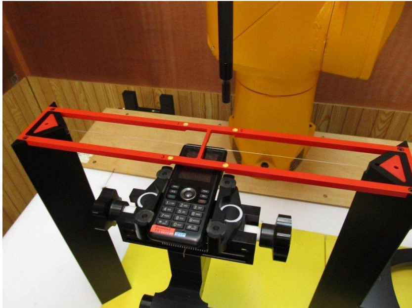
Figure 1a – HAC RF Emission Test Setup
