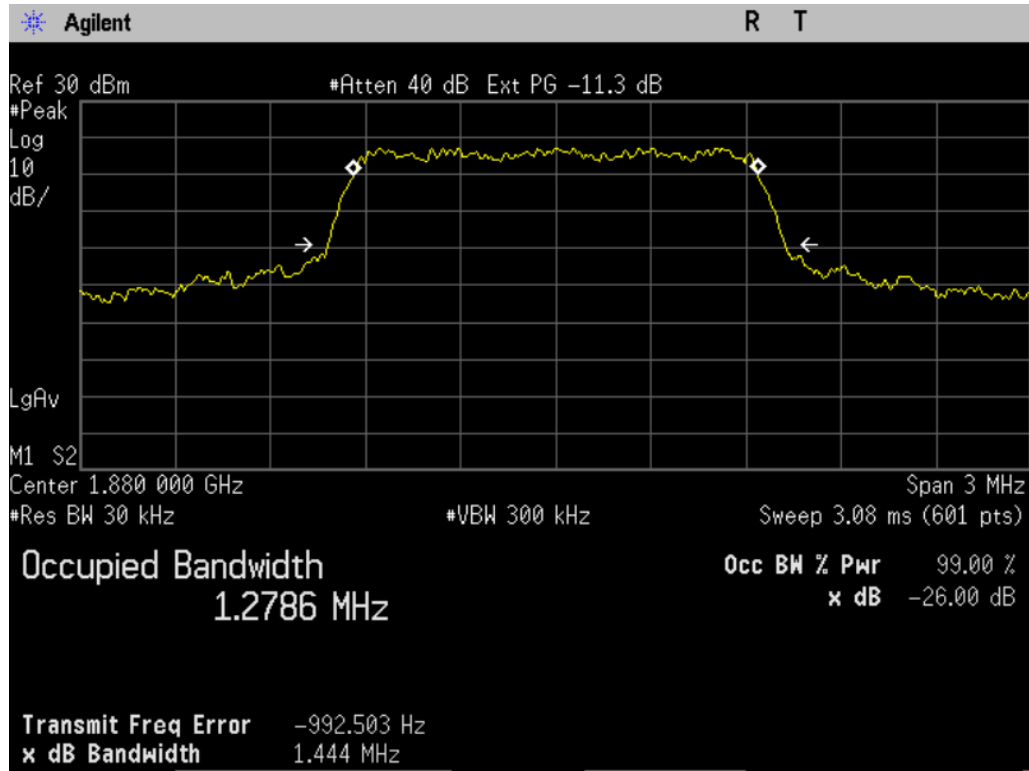
Figure 9-1 CDMA 1900 @ CH 600
