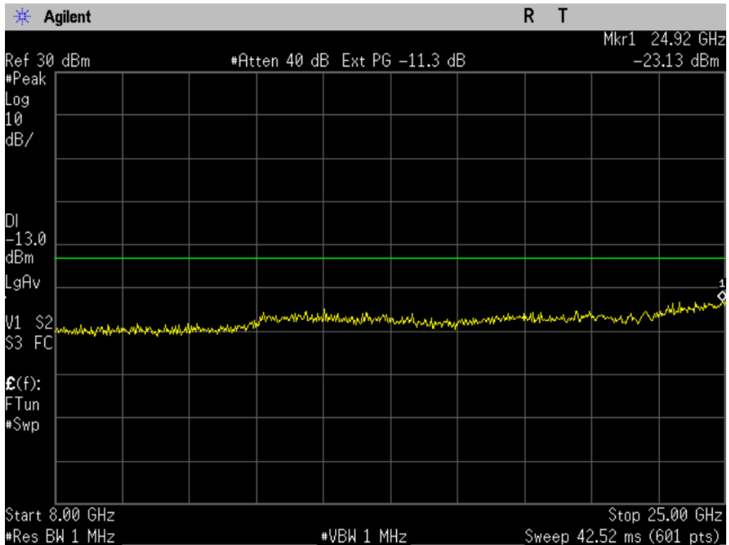
Figure 10-2b CDMA 1900 - Conducted Spurious Emission (CH 600)
