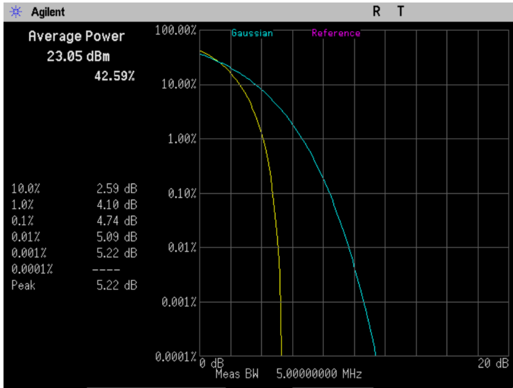
Figure 8-1 CCDF @ CH 600
