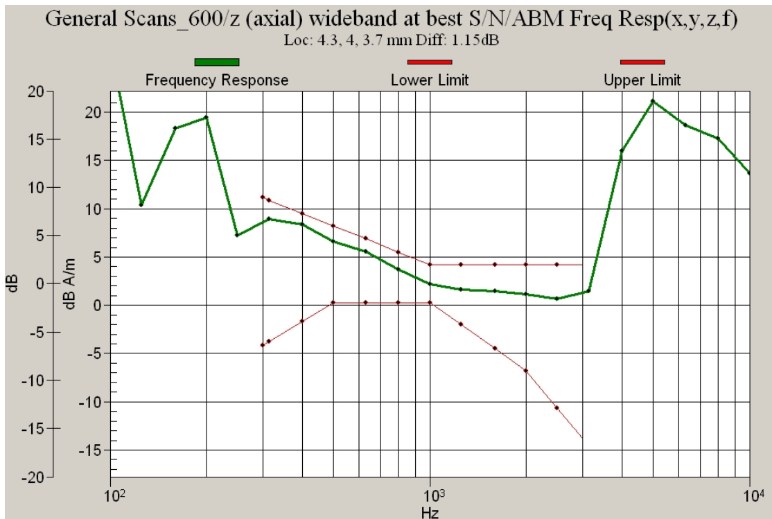
Figure 10.2a CDMA 1900 Channel 600 Frequency Response
