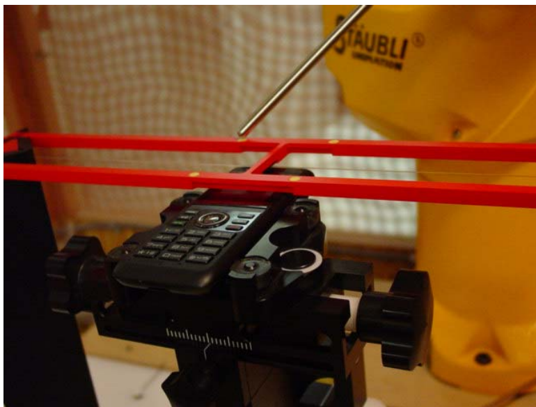
Figure 1b – HAC T-Coil Setup Photo
