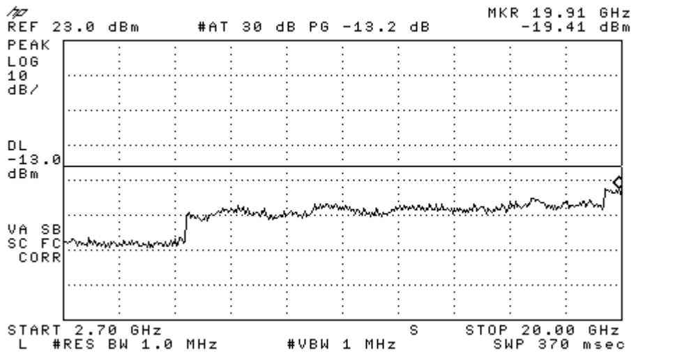
Figure 8-3b CDMA 1900 - Conducted Spurious Emission (CH 1175)
