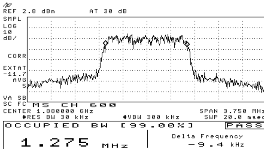
Figure 7-1 CDMA 1900 @ CH 600
