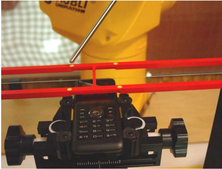
Figure 1a – HAC T-Coil Setup Photo
