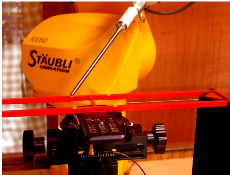
Figure 1a – HAC T-Coil Test Setup
