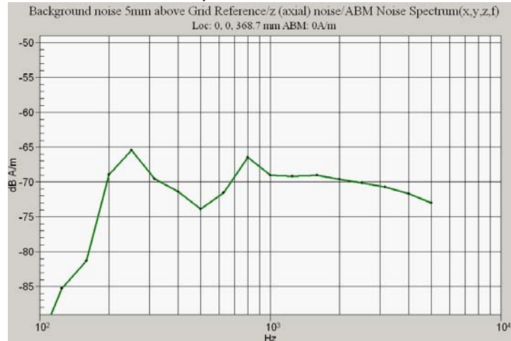
Ambient Noise Spectrum Plot Axial (z)
