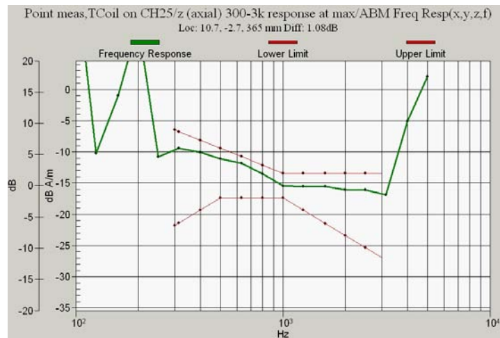
Figure 10.2a CDMA 1900 Channel 25 Frequency Response
