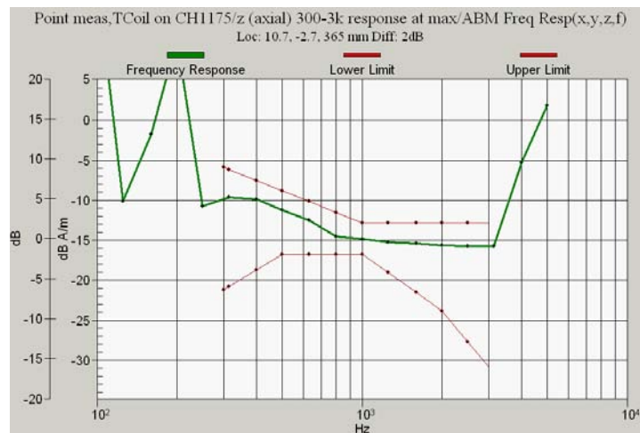
Figure 10.2c CDMA 1900 Channel 1175 Frequency Response
