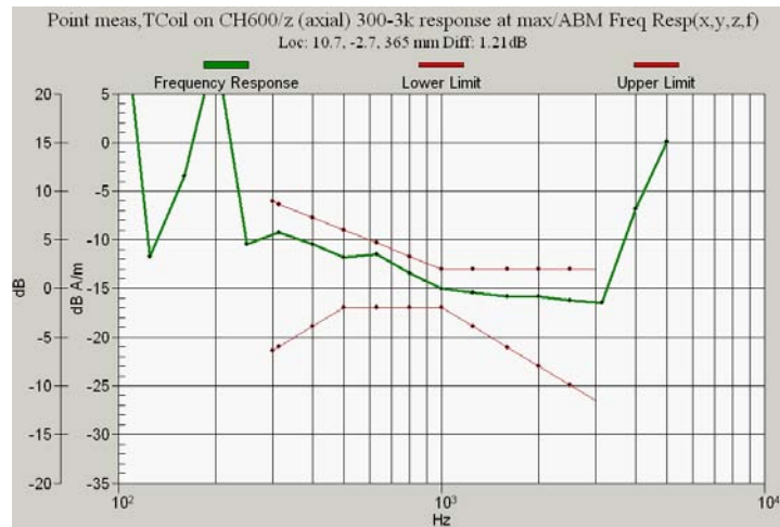
Figure 10.2b CDMA 1900 Channel 600 Frequency Response
