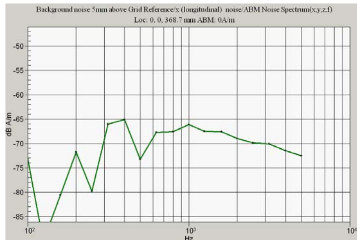
Ambient Noise Spectrum Plot Radial Longitudinal (x)
