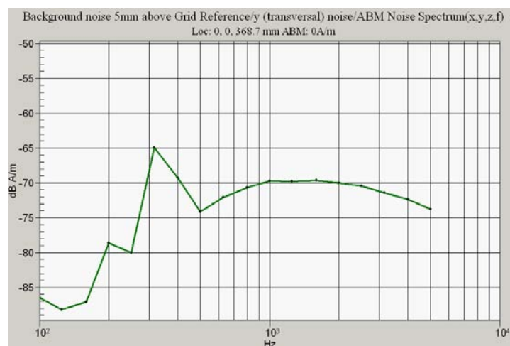
Ambient Noise Spectrum Plot Radial Transversal (y)
