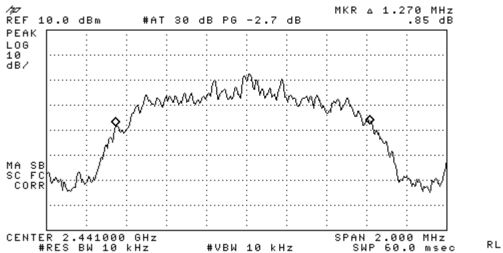
Figure 3-2c: 20 dB Bandwidth EDR 3Mbps, Channel 39.
