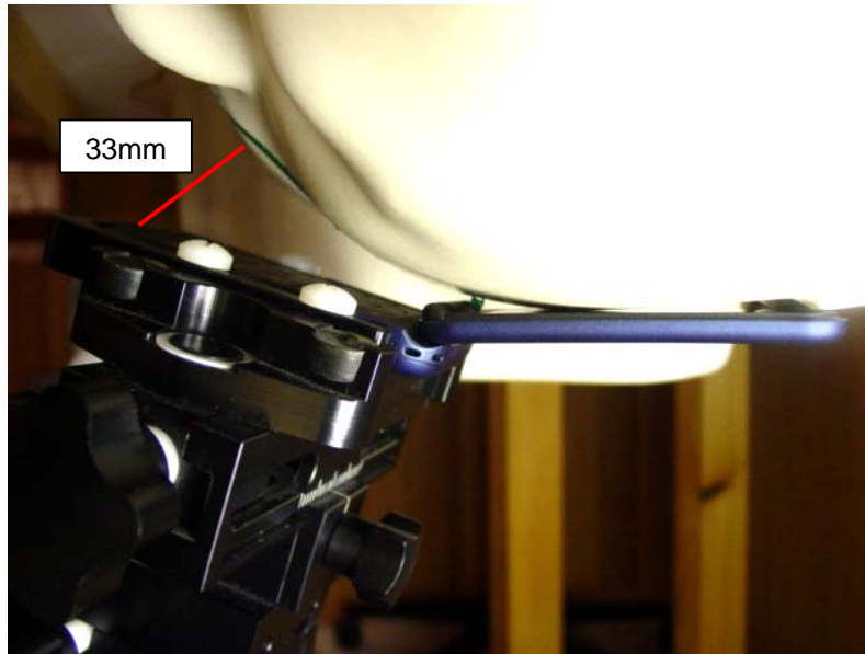
Figure 1 Phone against the head (cheek position)
