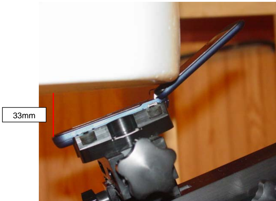
Figure 2 Phone against flat phantom (mouth position)
