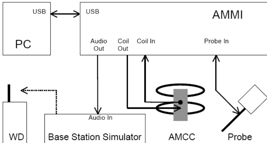
Figure 5.2b Setup Cabling
