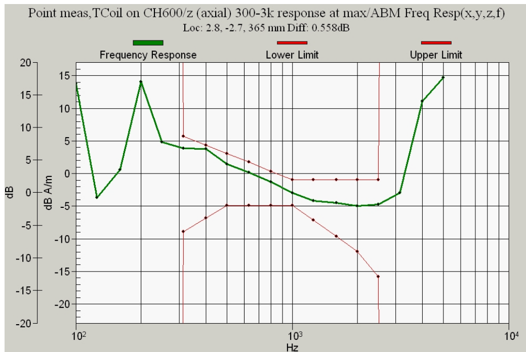
Figure 10.2b CDMA 1900 Channel 600 Frequency Response
