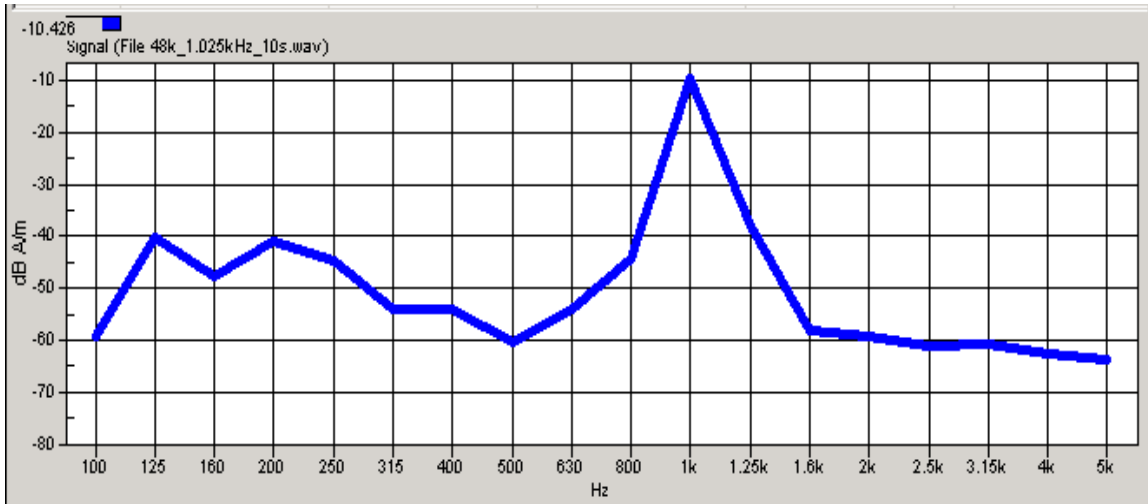
Figure 7.2a 1.025 KHz Voice signal spectrum
