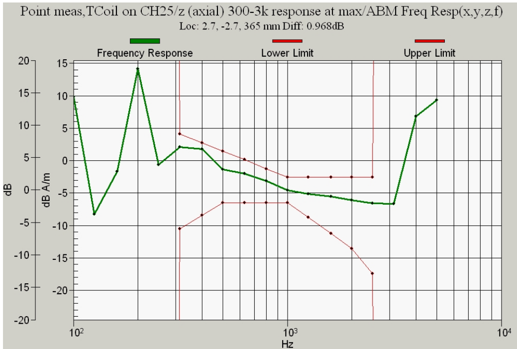
Figure 10.2a CDMA 1900 Channel 25 Frequency Response
