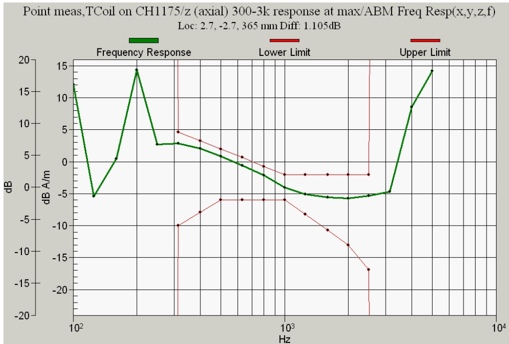
Figure 10.2c CDMA 1900 Channel 1175 Frequency Response
