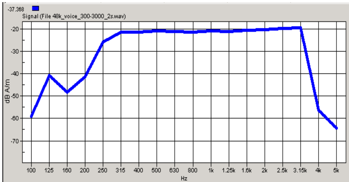
Figure 7.2b Broadband signal spectrum
