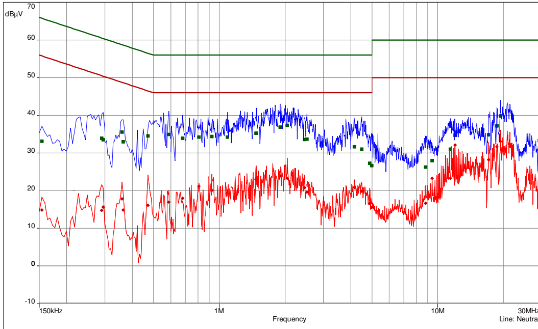
CISPR 22/CISPR22B
