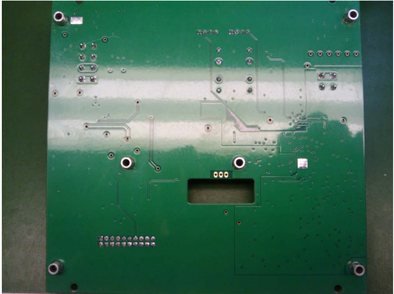
Control Board PCB for AMP460-1 BACK
