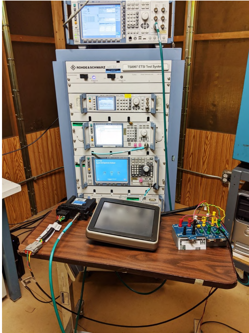
Figure 1: Equipment Under Test – Radiated Emissions – Antenna Port Conducted Measurements
