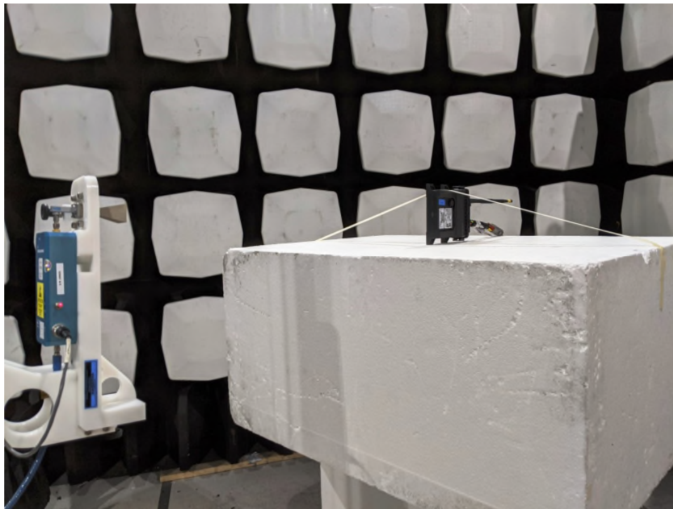
Figure 8: Equipment Under Test – Radiated Emissions >18GHz
