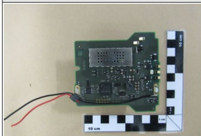
RADIATED SAMPLE
