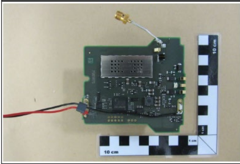
CONDUCTED SAMPLE
