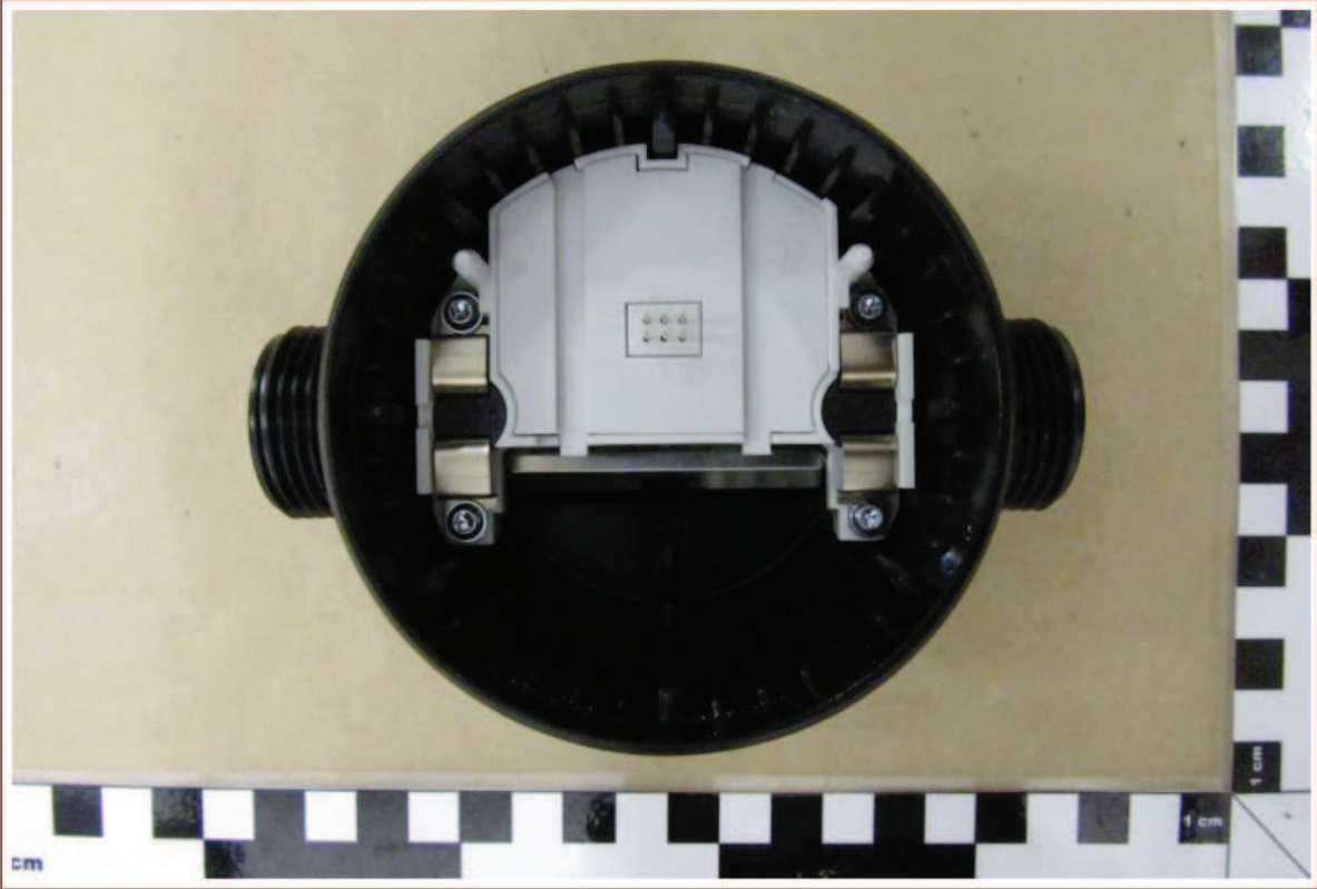
EUT, flow part internal picture
