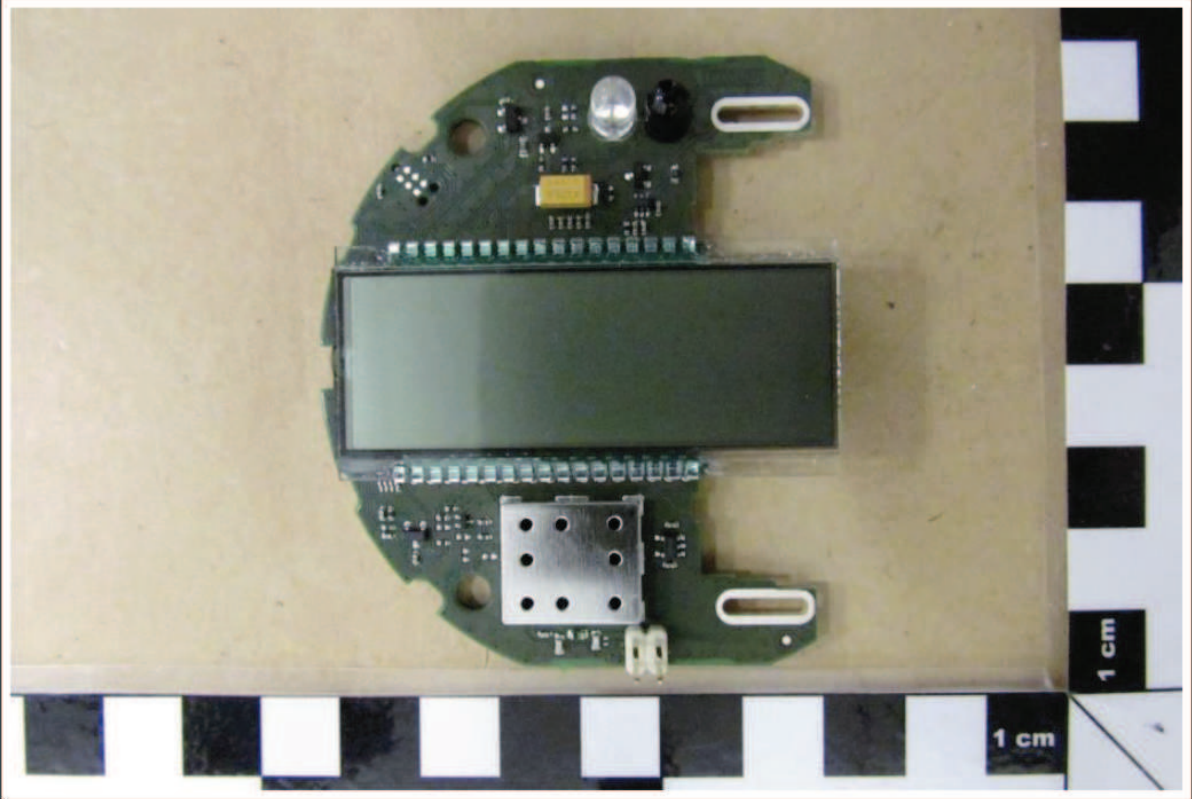
PCB, 55501810 radiated_sample
