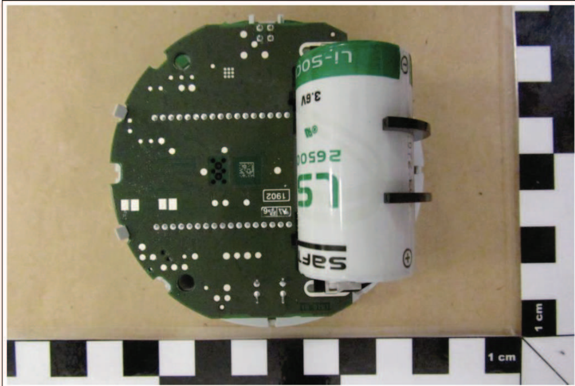
PCB, 55501810 assembly with battery bottom view
