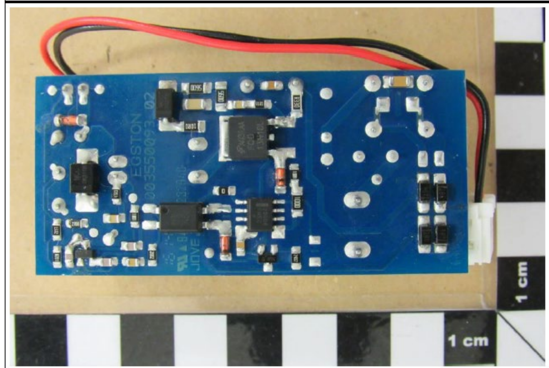
24 VAC smps supply bottom view (6020000400000 A4)
