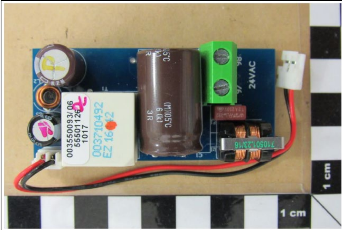
24 VAC smps supply top view (6020000400000 A4)
