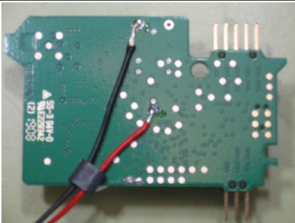
55501605revF1_Back
