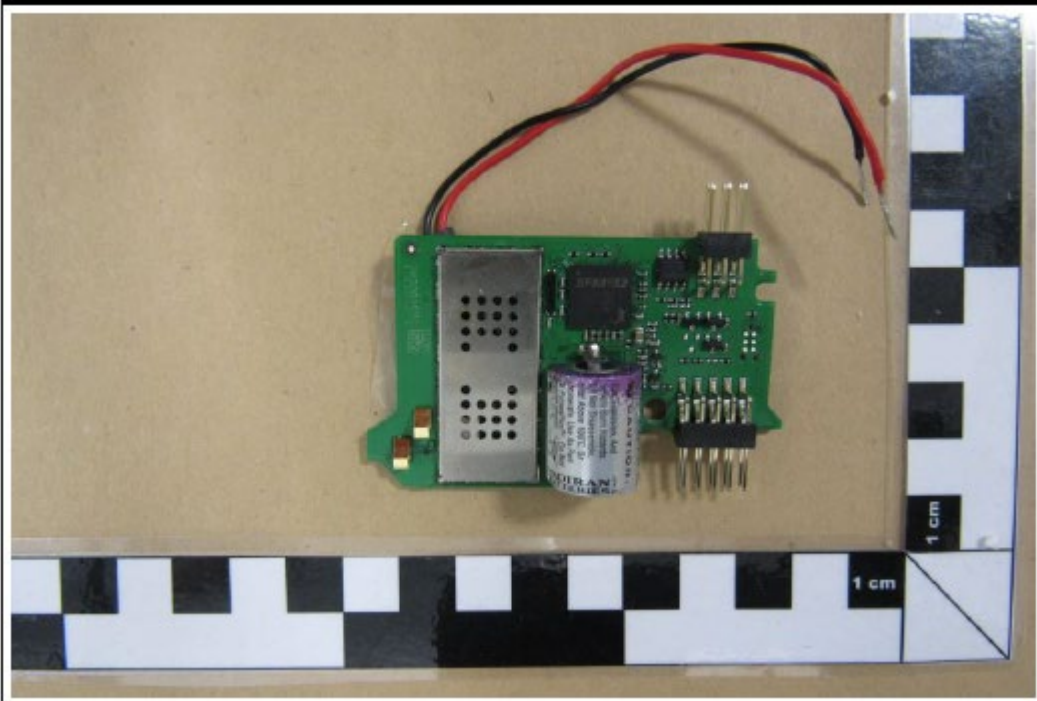
FlowIQ 2250 RF-PCB
