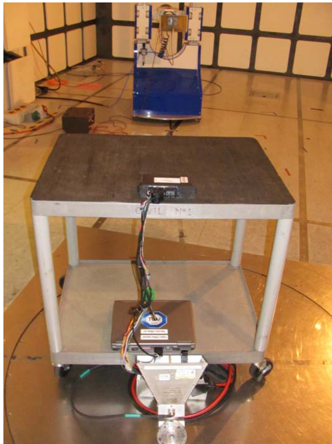
Radiated Emissions 1GHz-18GHz – FCC 24 Internal Antenna
