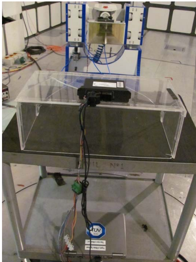
Radiated Emissions 17GHz-18GHz – FCC 15.247 Internal Antenna
