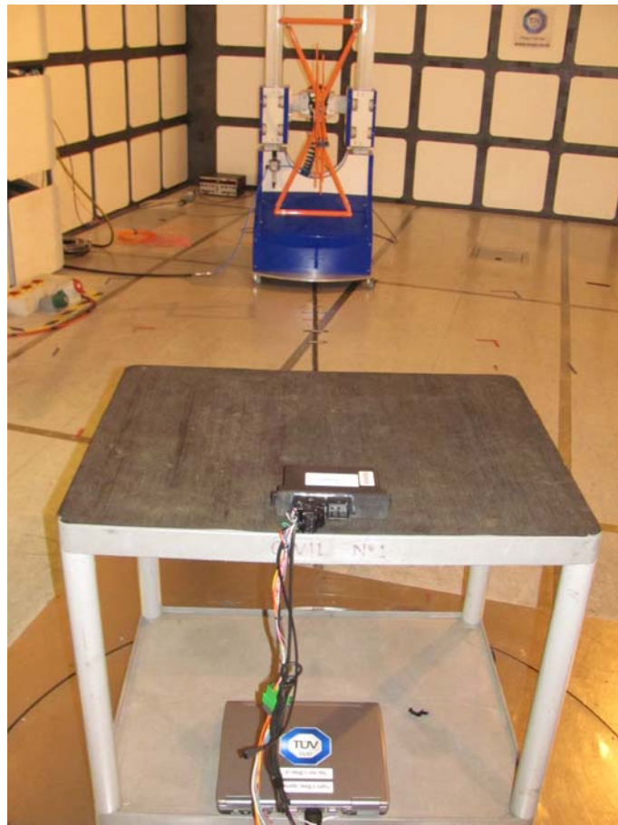
Radiated Emissions 30MHz-1GHz – FCC 15 B & 15.247 Internal Antenna
