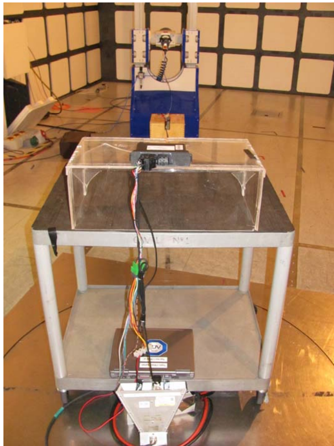
Radiated Emissions 18GHz-20GHz – FCC 24 Internal Antenna
