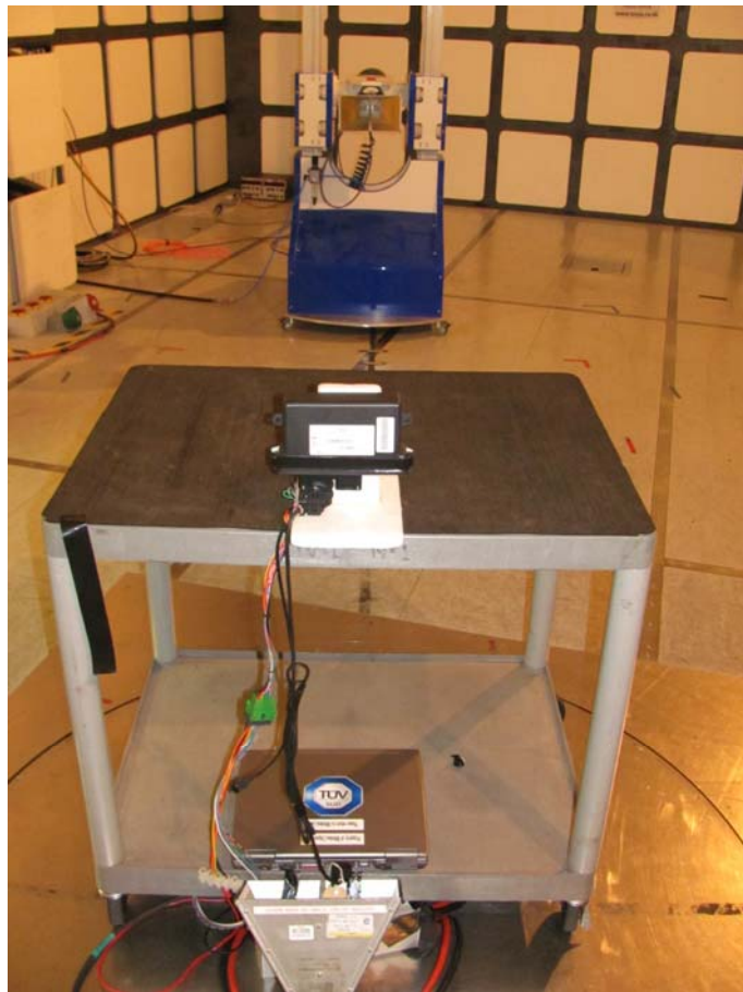
Radiated Emissions 1GHz-9GHz – FCC 22 Internal Antenna
