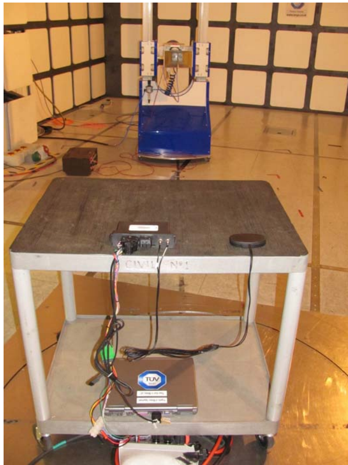
Radiated Emissions 1GHz-13GHz – FCC 15 B External Antenna
