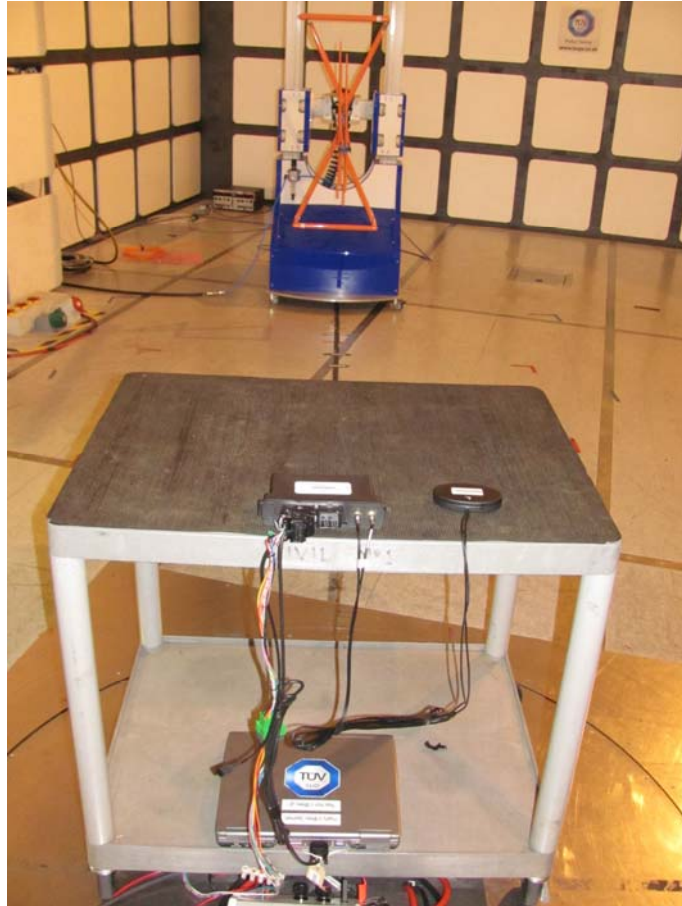
Radiated Emissions 30MHz-1GHz – FCC 15 B External Antenna
