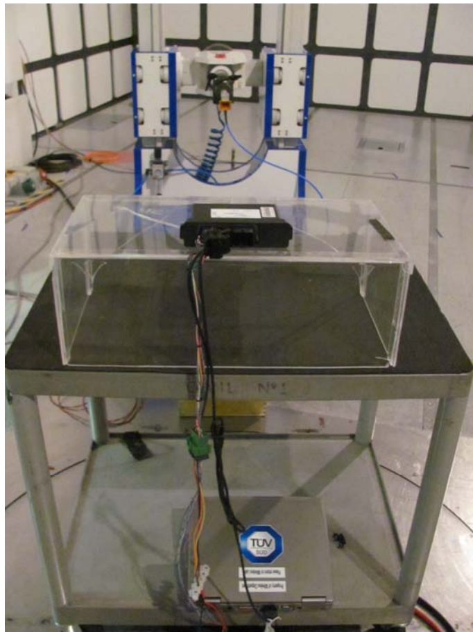
Radiated Emissions 18GHz-25GHz – FCC 15.247 Internal Antenna
