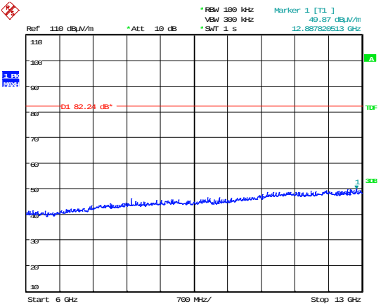
Figure 10 – Intermodulation GSM850 and Bluetooth Classic (6 GHz to 13 GHz); Channel Top.
