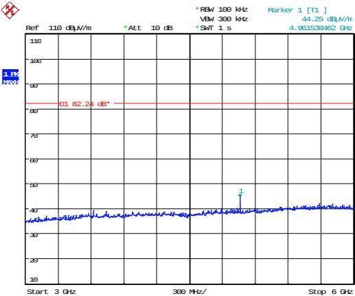
Figure 9 – Intermodulation GSM850 and Bluetooth Classic (3 GHz to 6 GHz); Channel Top.
