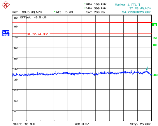
Figure 12 – Intermodulation GSM1900 and Bluetooth LE (18 GHz to 25 GHz); Channel Top.
