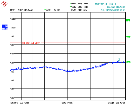
Figure 11 – Intermodulation GSM1900 and Bluetooth LE (13 GHz to 18 GHz); Channel Top.
