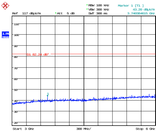
Figure 9 – Intermodulation GSM1900 and Bluetooth LE (3 GHz to 6 GHz); Channel Top.
