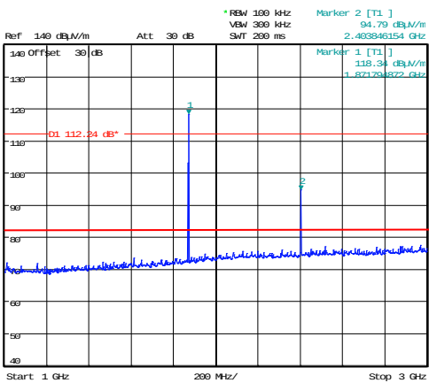
Figure 2 – Intermodulation GSM1900 and Bluetooth Classic (1 GHz to 3 GHz); Channel Bottom.
