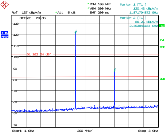
Figure 2 – Intermodulation GSM1900 and Bluetooth LE (1 GHz to 3 GHz); Channel Bottom.
