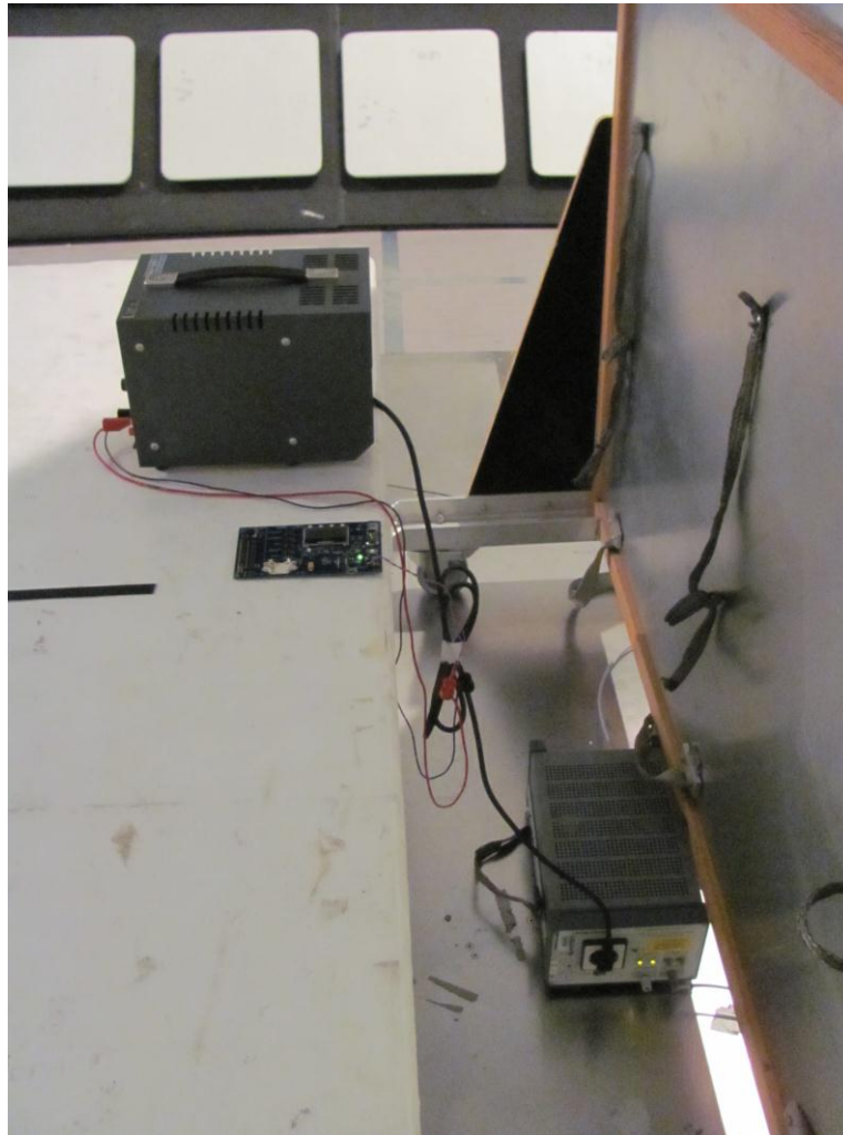
Figure 3: Setup for conducted emissions
