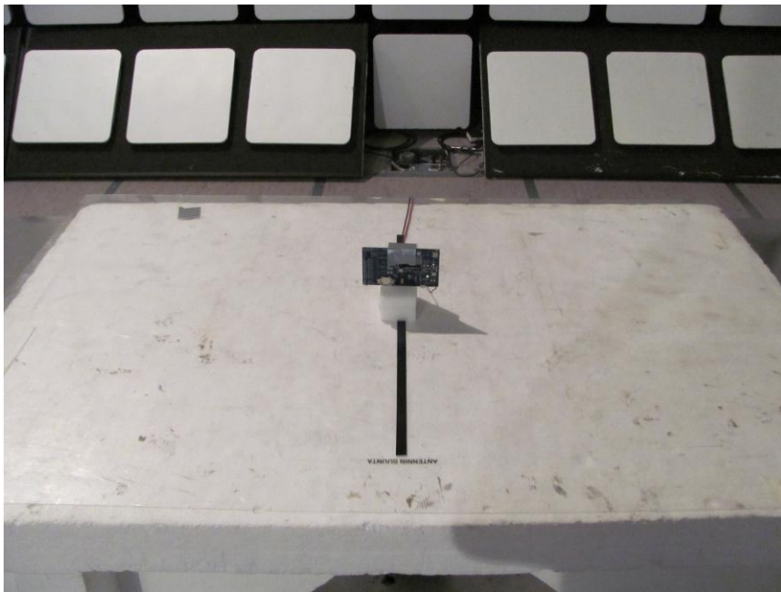
Figure 2: Setup for radiated emissions
