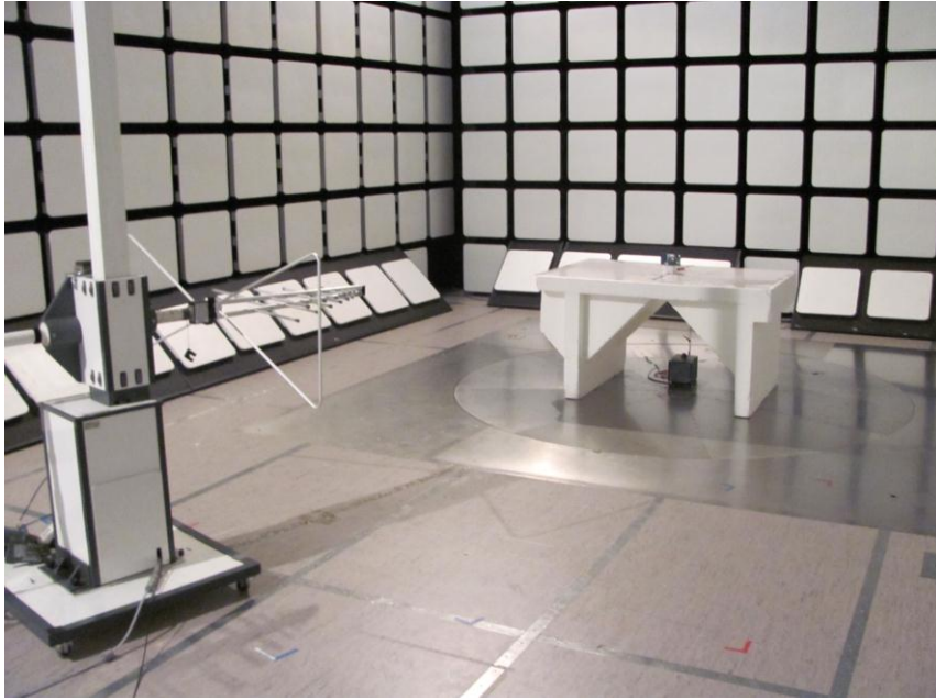
Figure 1: Setup for radiated emissions
