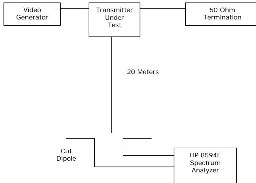
Figure 4-11. Test Setup for Measuring Radiated Emissions
