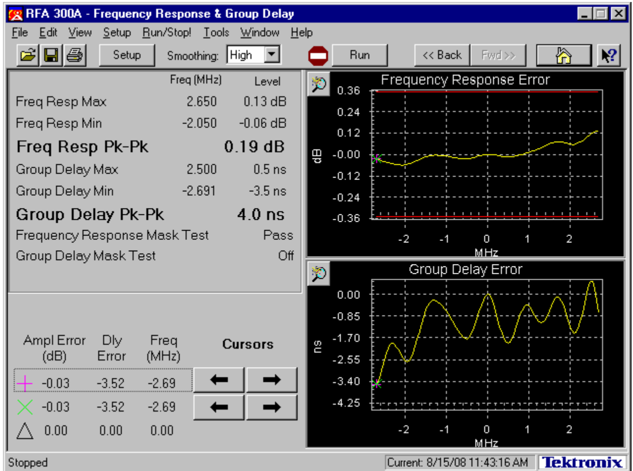
Figure 4B-4. Frequency Response Plot
