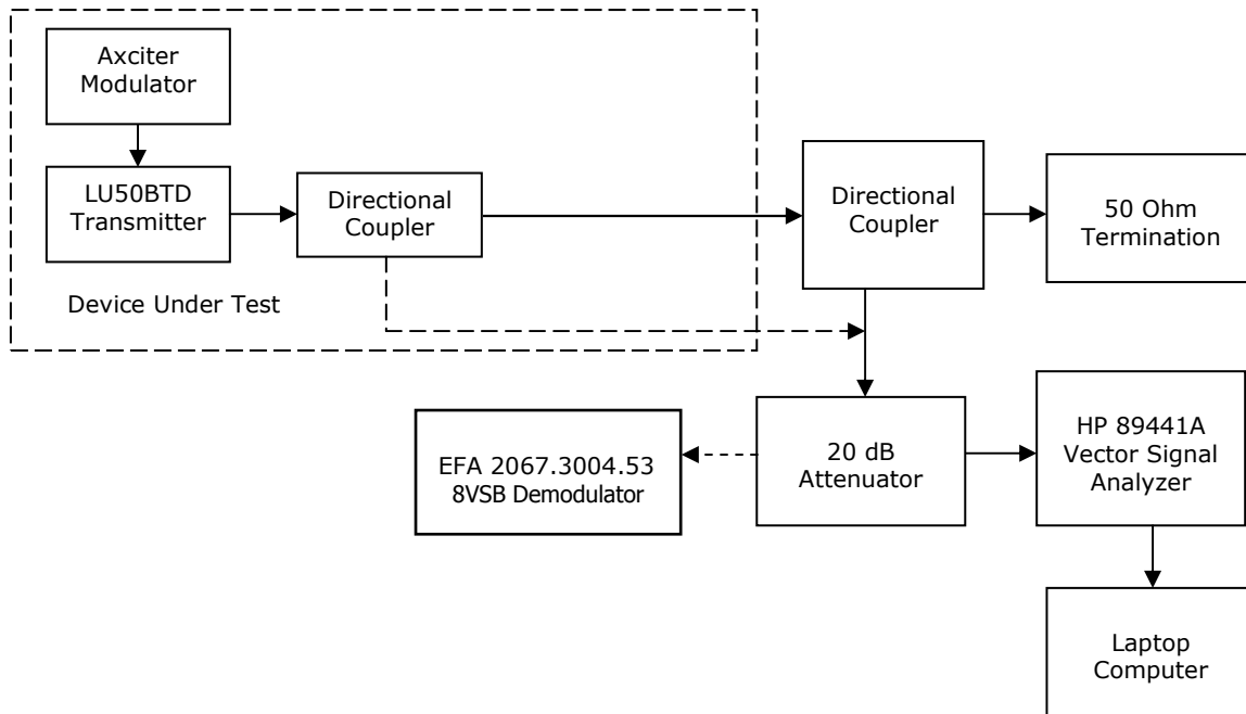
Figure 4B-2. Typical Demodulation Test Setup
