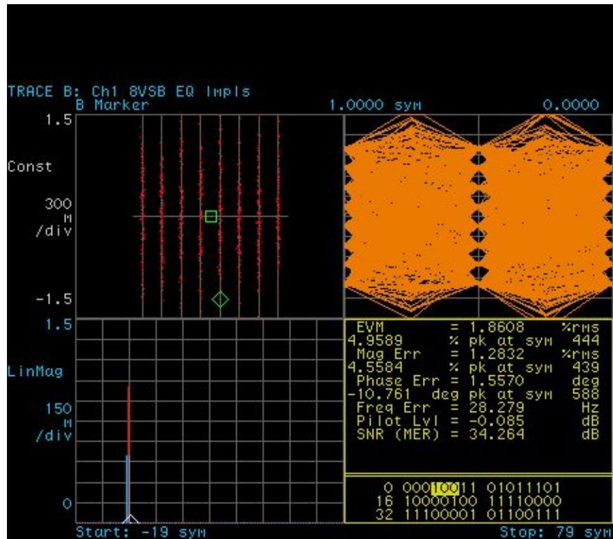
Figure 4B-3. Constellation Diagram
