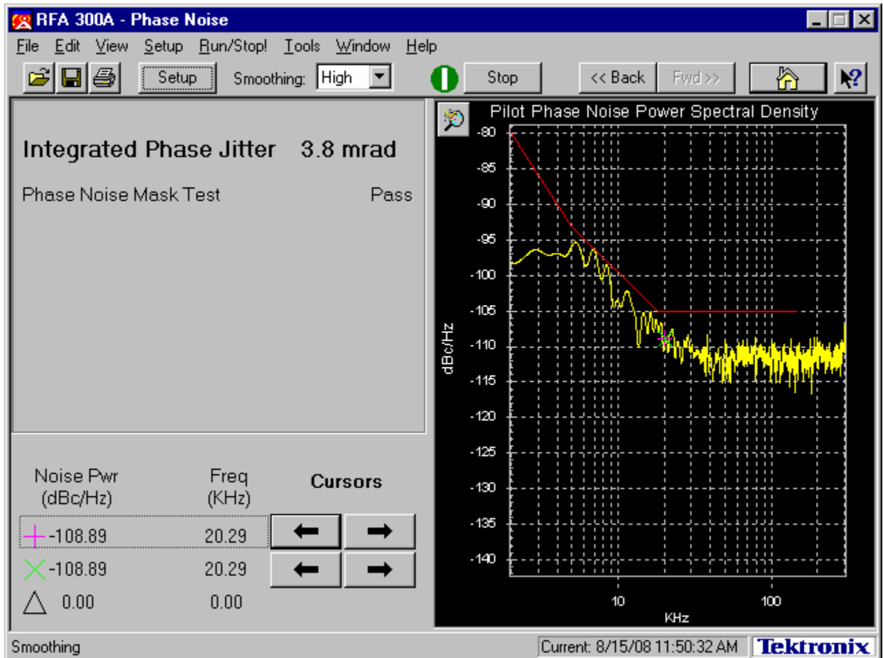
Figure 4B-6. Phase Noise Plot
