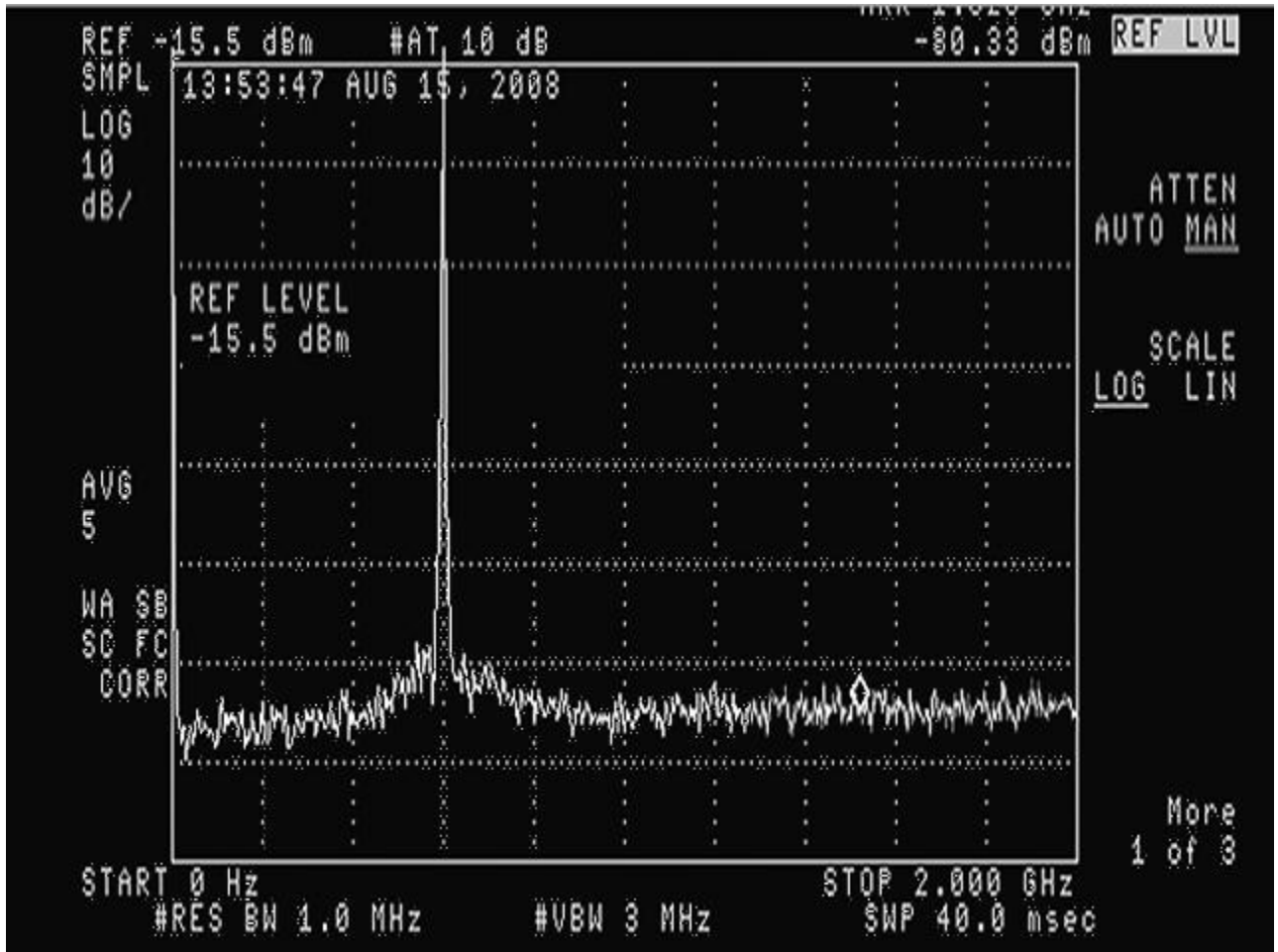
Figure 4B-8A. Out of Band Emissions Plot (Pre-Filter)
