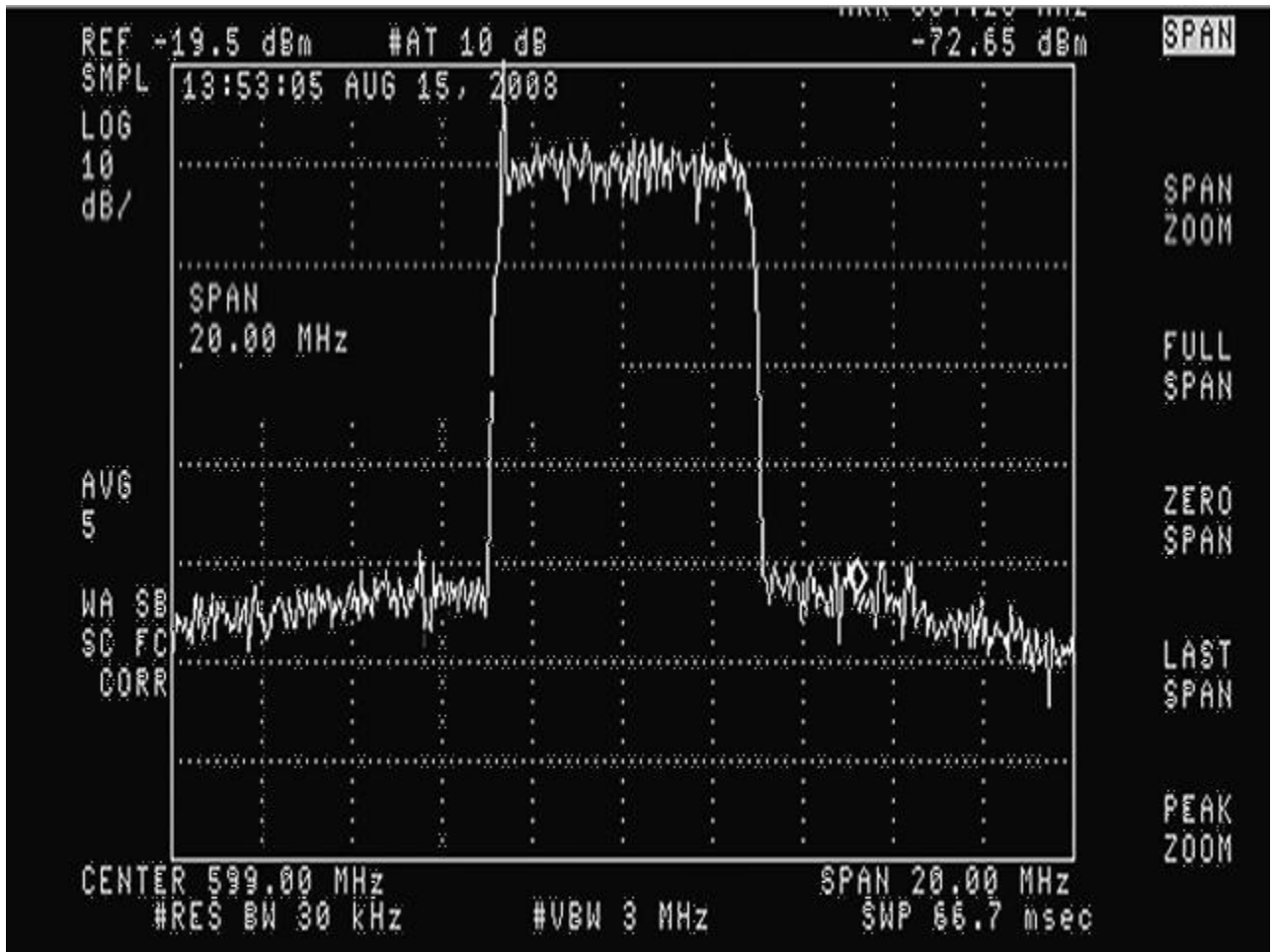
Figure 4B-7. Channel Occupied Bandwidth (Pre-Filter)
