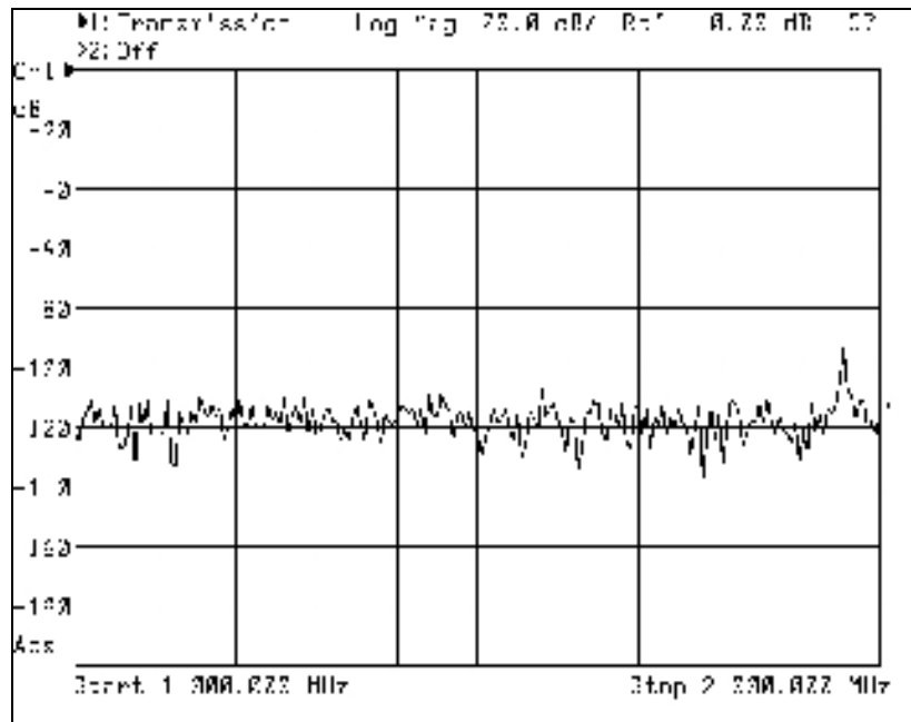
Figure 4B-8C. Simple Mask Filter Harmonic Rejection
