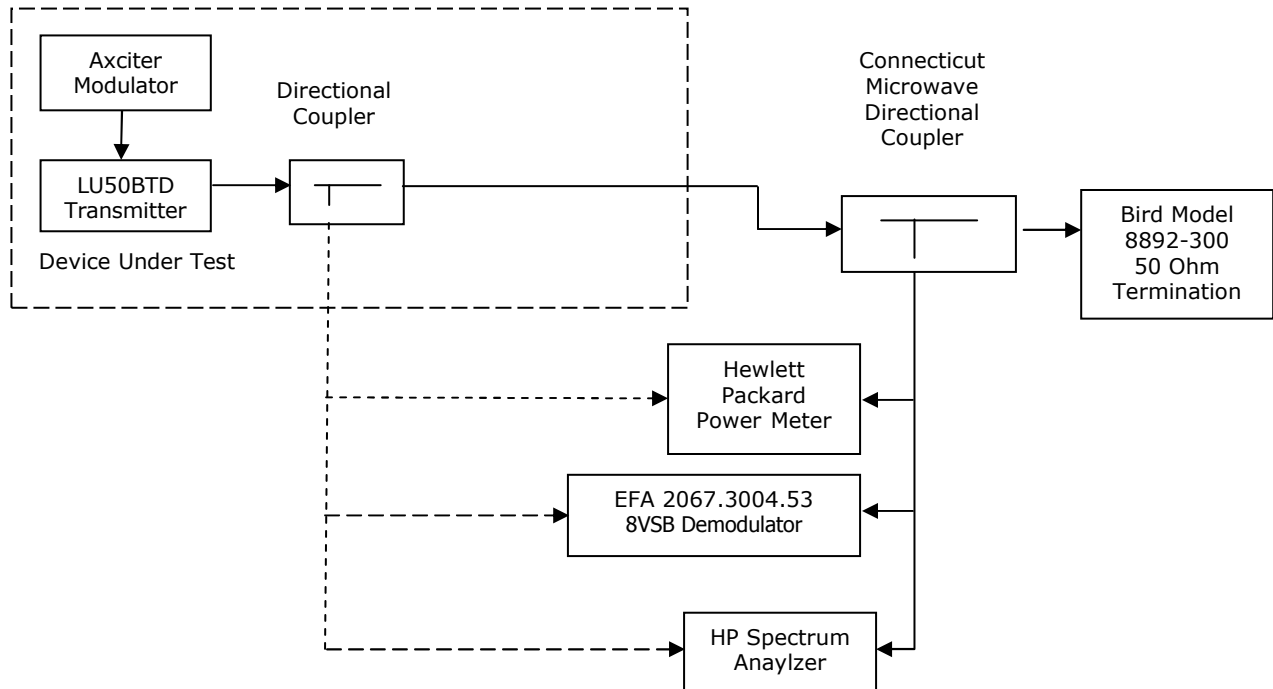
Figure 4B-1. Test Equipment Setup for RF Power Measurements
