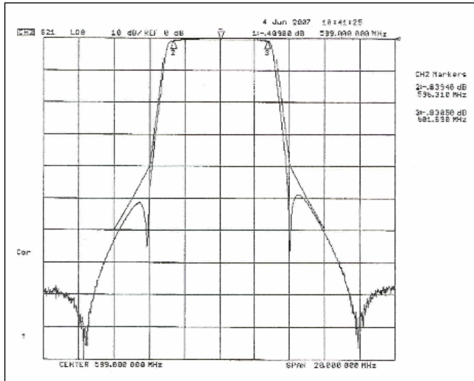
Figure 4B-8D. Bandpass Filter Response (Stringent Mask)
