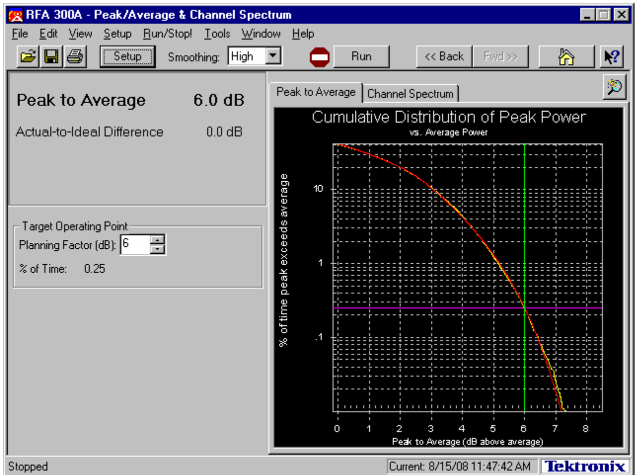
Figure 4B-5. Peak to Average Plot
