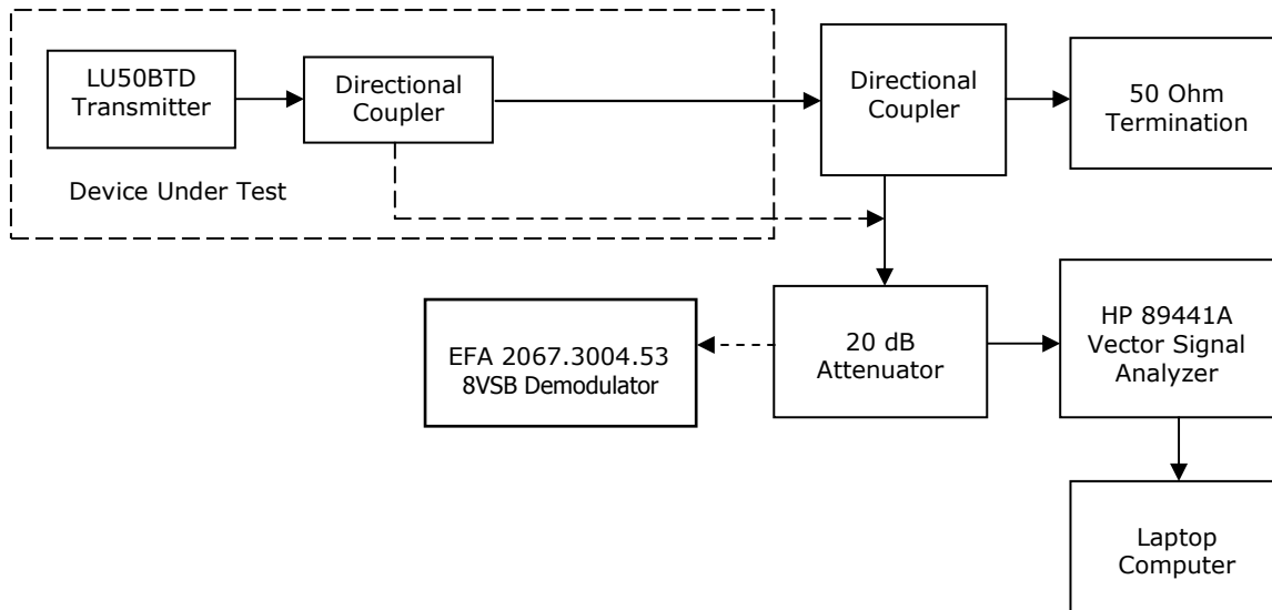
Figure 4A-2. Typical Demodulation Test Setup
