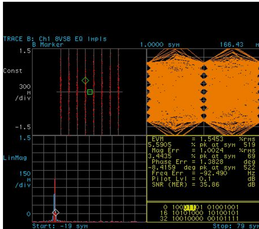
Figure 4A-3. Constellation Diagram
