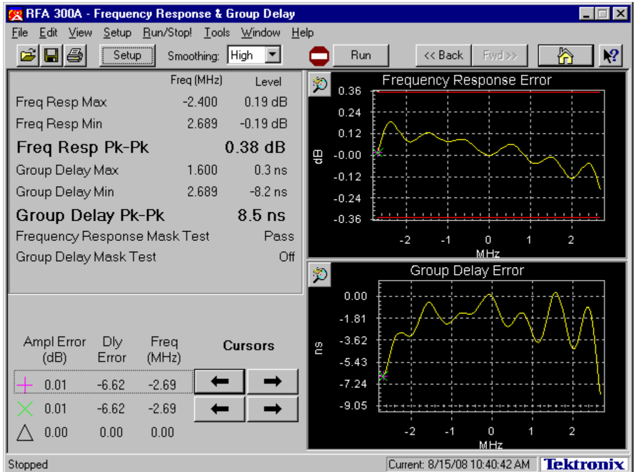
Figure 4A-4. Frequency Response Plot
