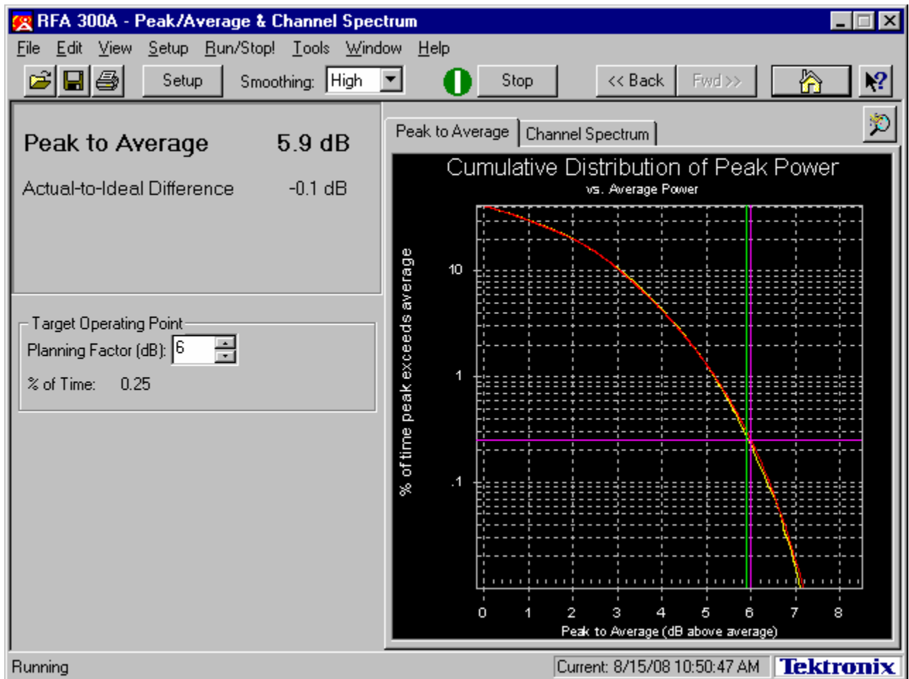
Figure 4A-5. Peak to Average Plot
