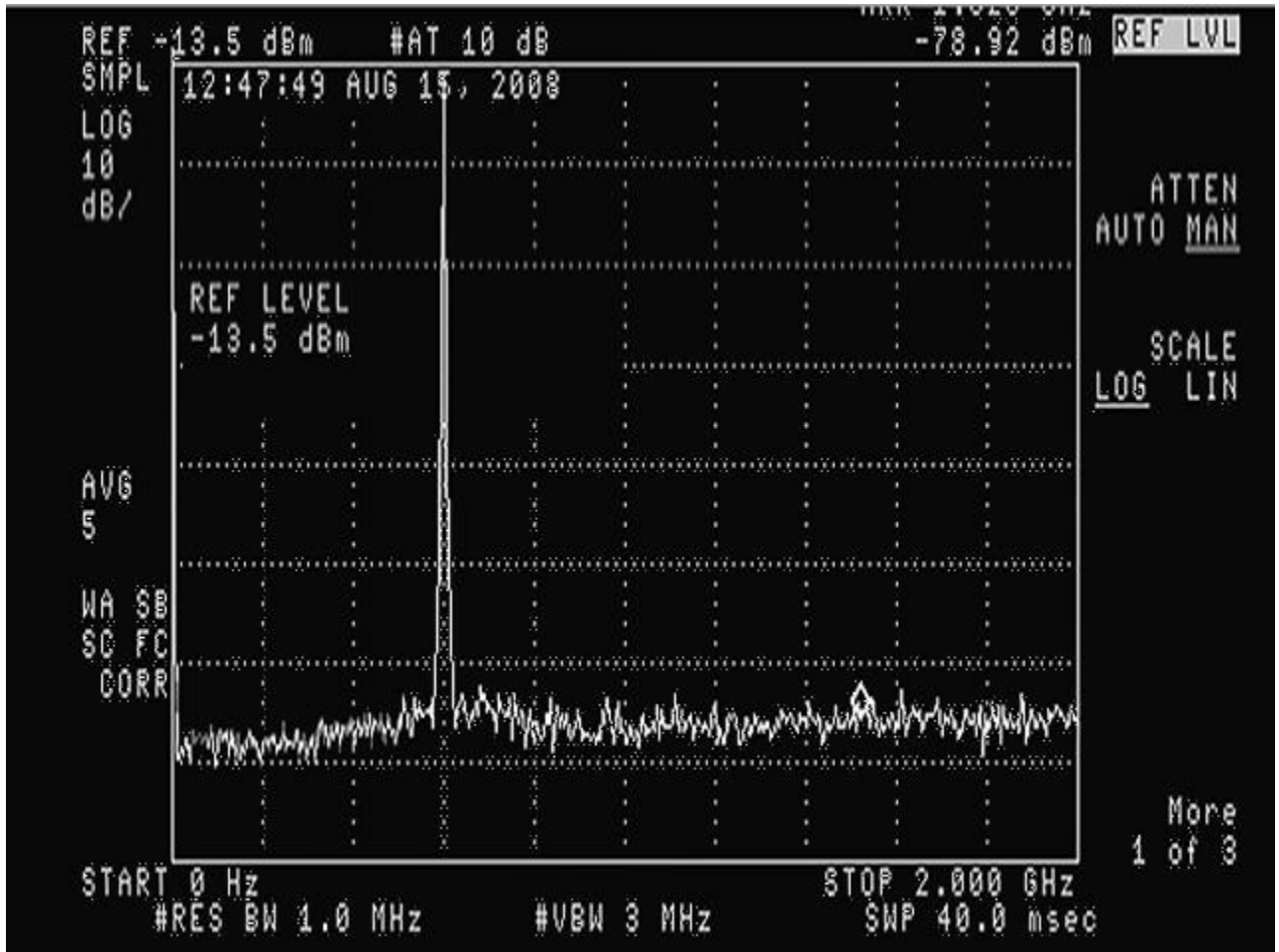
Figure 4A-8A. Out of Band Emissions Plot (Pre-Filter)
