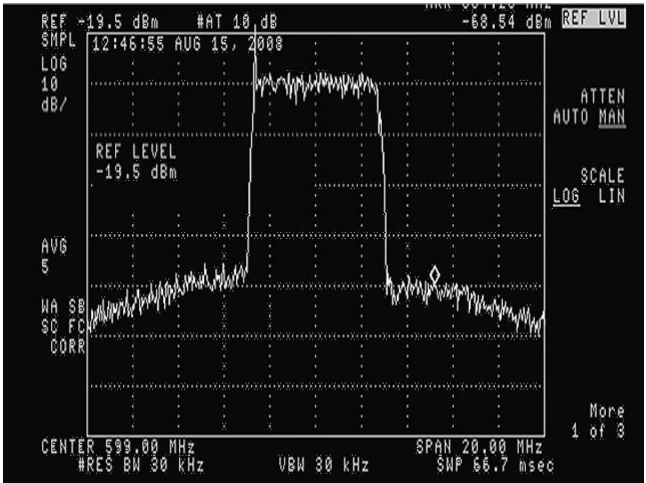
Figure 4A-7. Channel Occupied Bandwidth (Pre-Filter)
