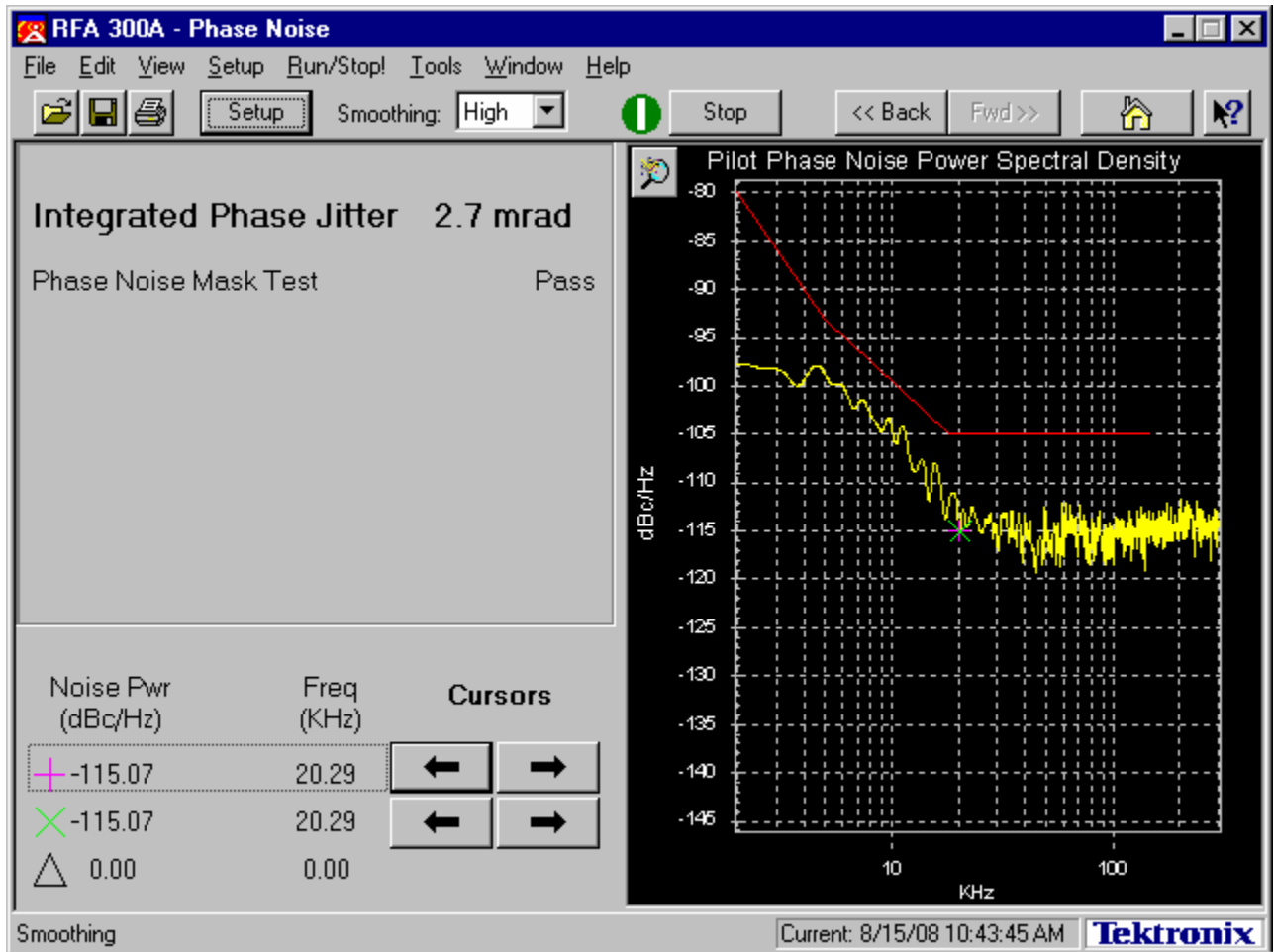
Figure 4A-6. Phase Noise Plot
