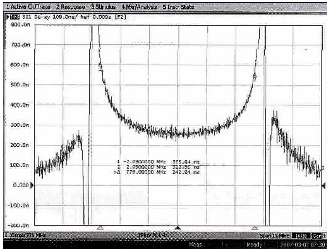
Figure 4-8F. Group Delay
