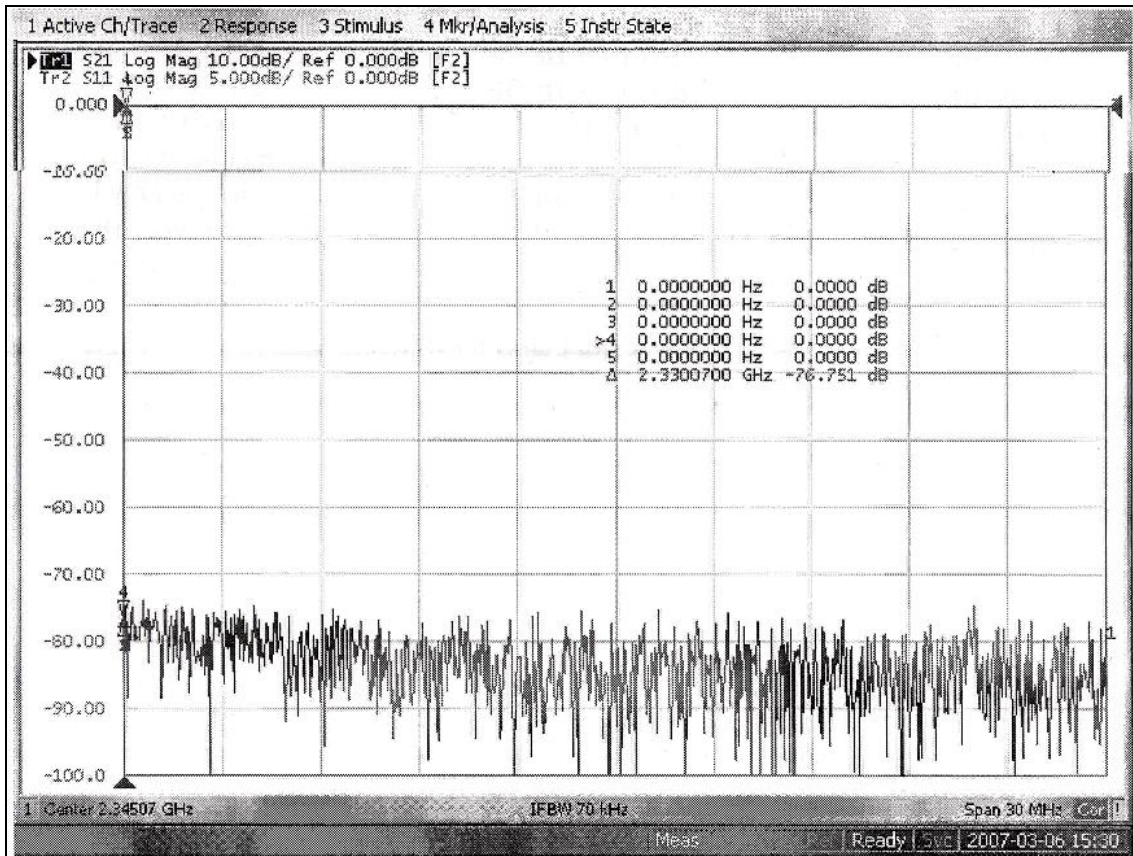
Figure 4-8J. Third Harmonic
