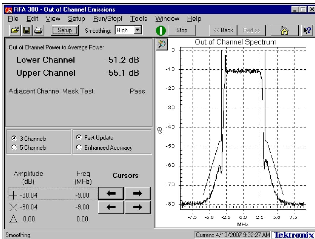
Figure 4-8K. Out of Band Emissions Plot (Post-Filter)
