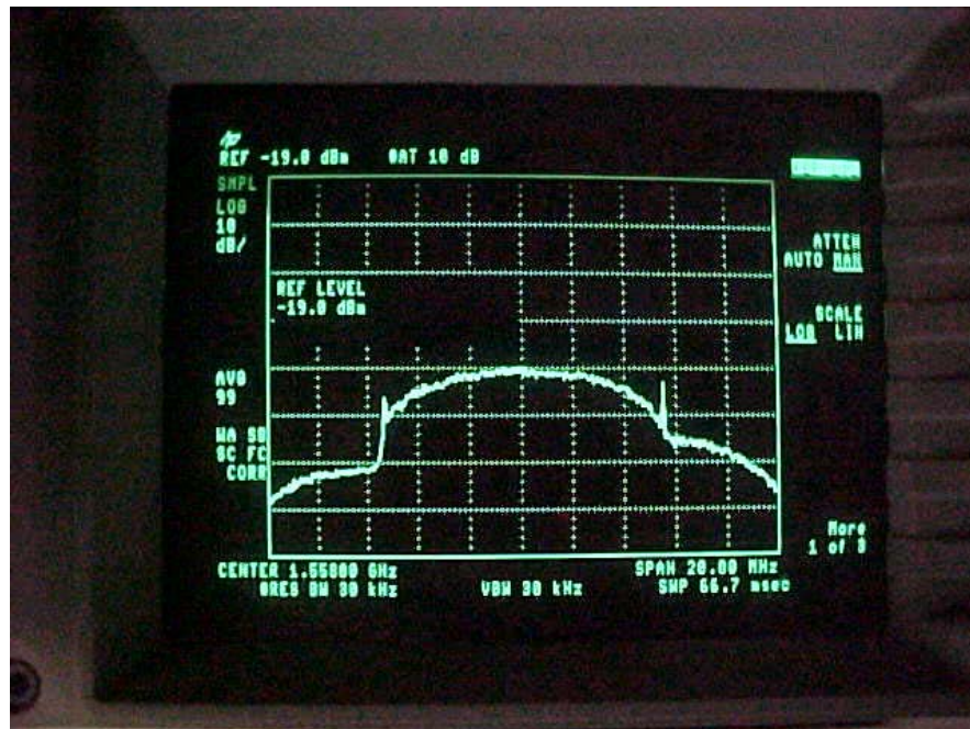
Figure 4-8B. Second Harmonic (1558.00 MHz) = -59.0 dBm (Pre-Filter)
