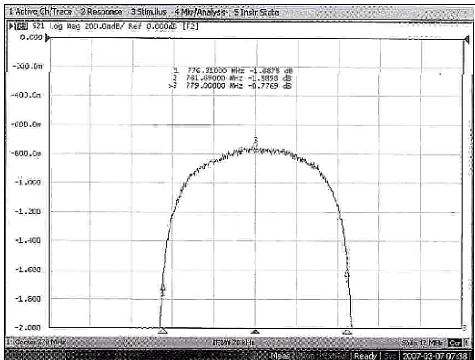
Figure 4-8E. Insertion Loss
