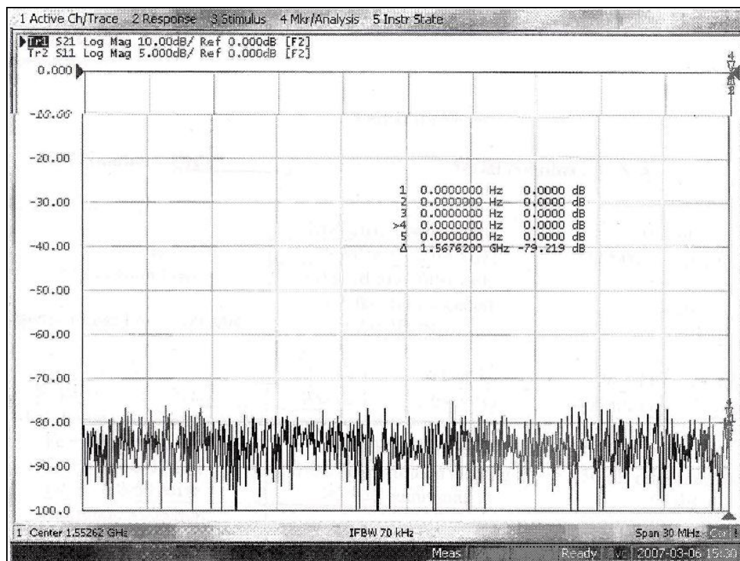
Figure 4-8I. Second Harmonic
