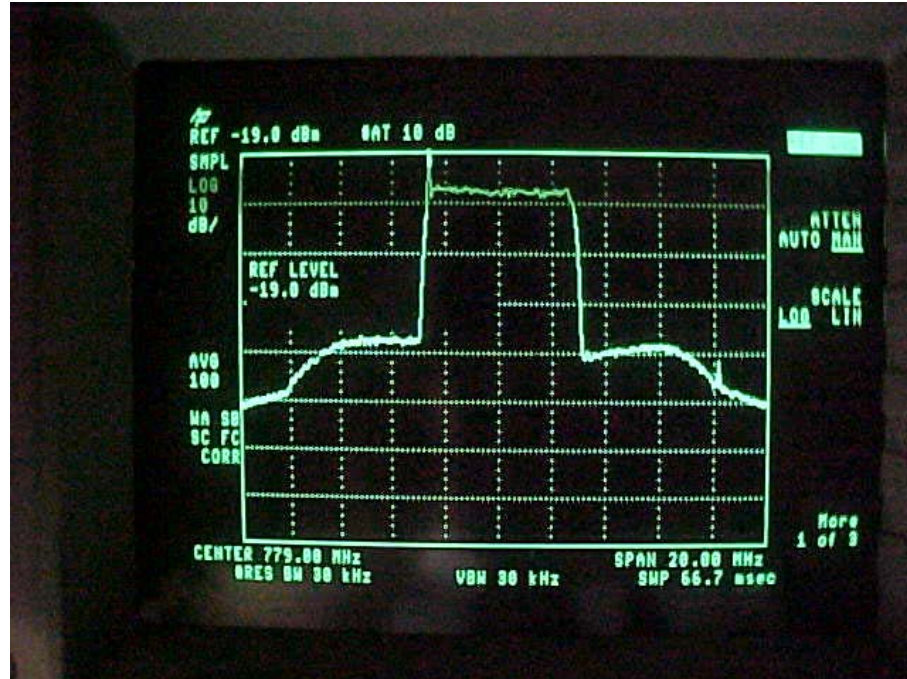
Figure 4-8A. Reference (779.00 MHz) = -19.0 dBm (Pre-Filter)
