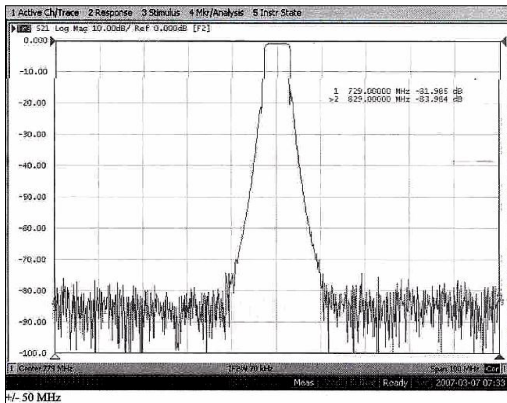
Figure 4-8H. \pm 50 MHz
