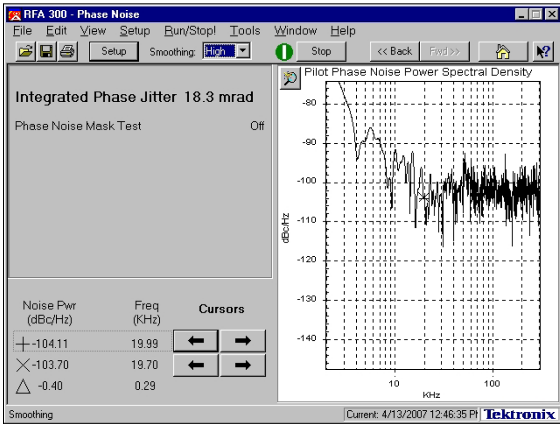
Figure 4-6. Phase Noise Plot
