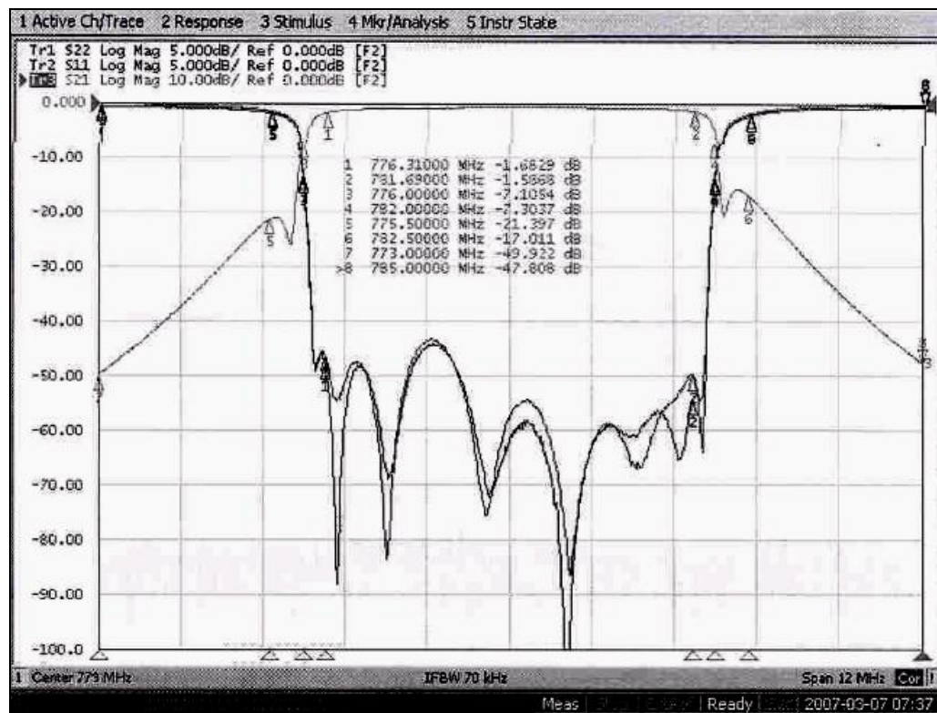
Figure 4-8G. Filter Response and Port Match
