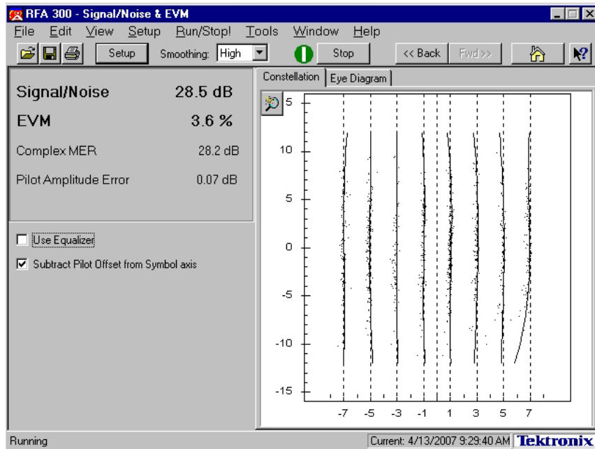
Figure 4-3. Constellation Diagram
