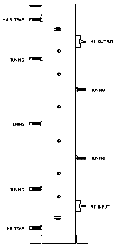
Figure 5-2. Bandpass Filter
