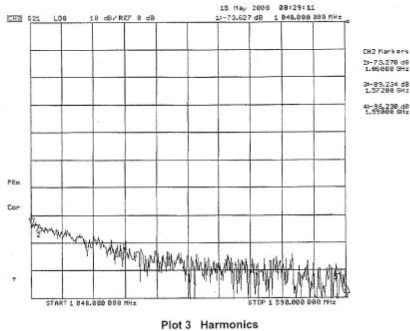
Figure 4B-8D. Harmonics
