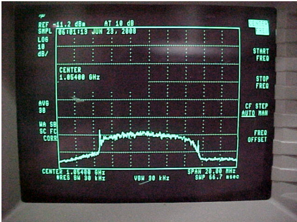
Figure 4B-8B. Second Harmonic 1054 MHz) = -58 dBm (Pre-Filter)
