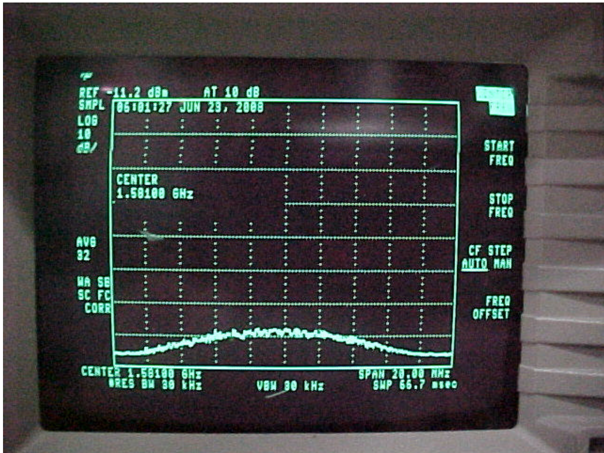
Figure 4B-8C. Third Harmonic (1581 MHz) = -68 dBm (Pre-Filter)
