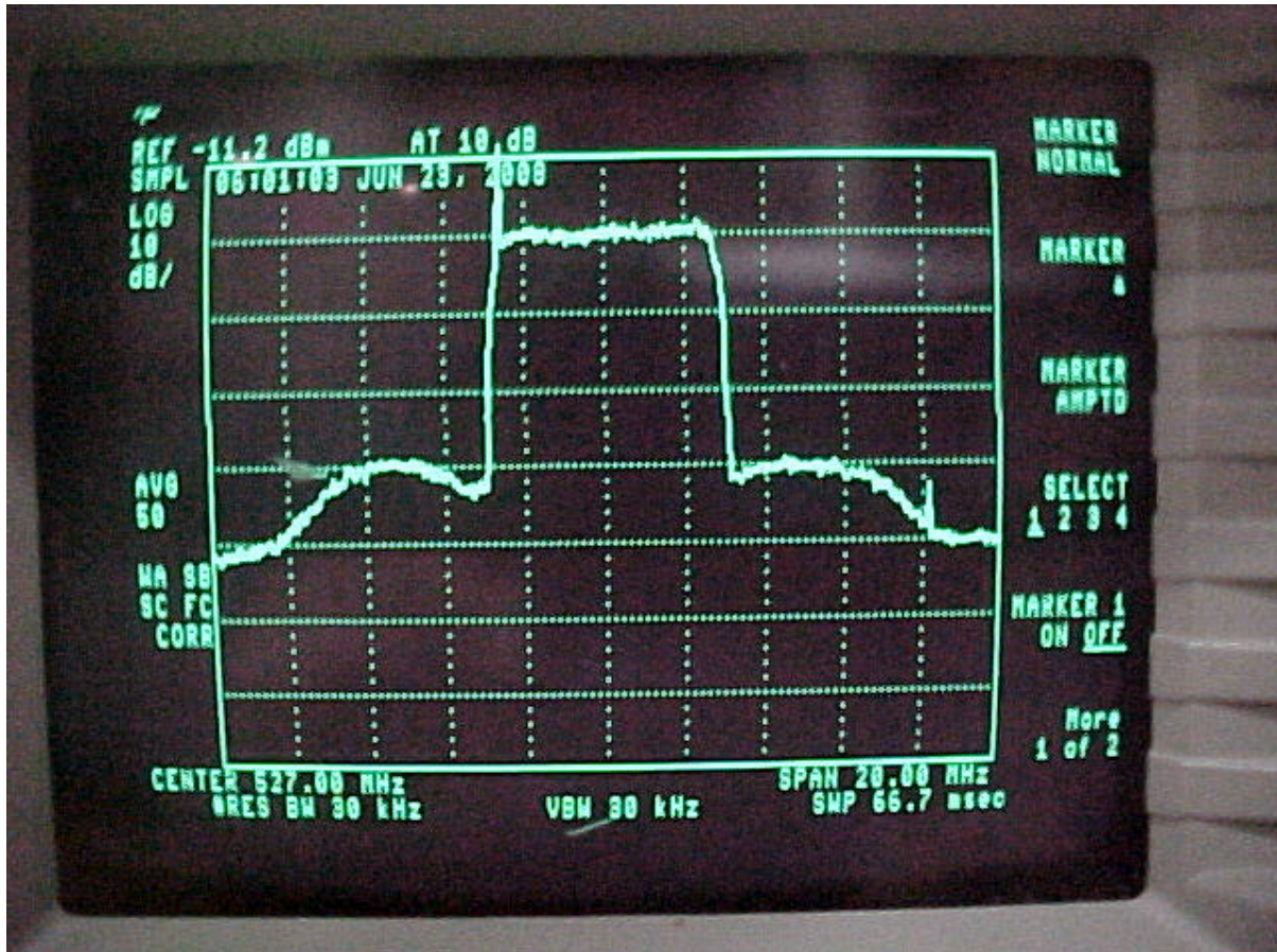
Figure 4B-8A. Reference (527 MHz) = 0 dBm (Pre-Filter)
