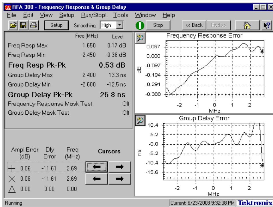
Figure 4B-4. Frequency Response and Group Delay Plots
