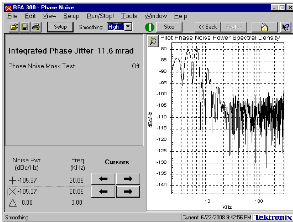
Figure 4B-6. Phase Noise Plot
