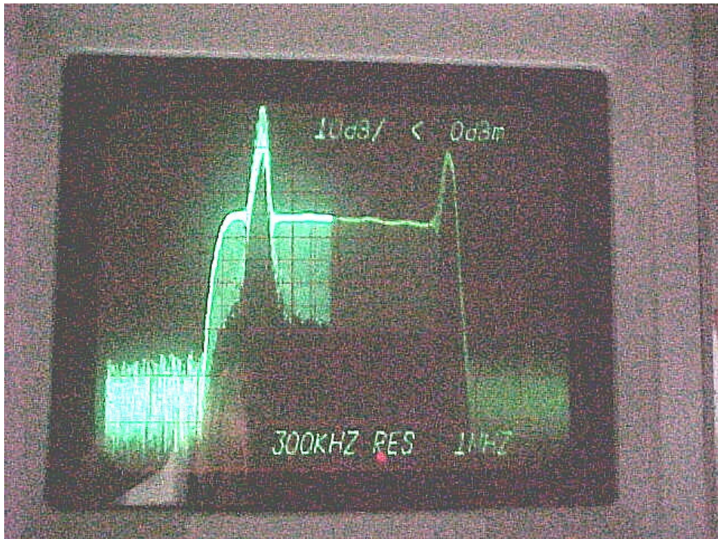
Figure 4-7. Channel-Occupied Bandwidth
