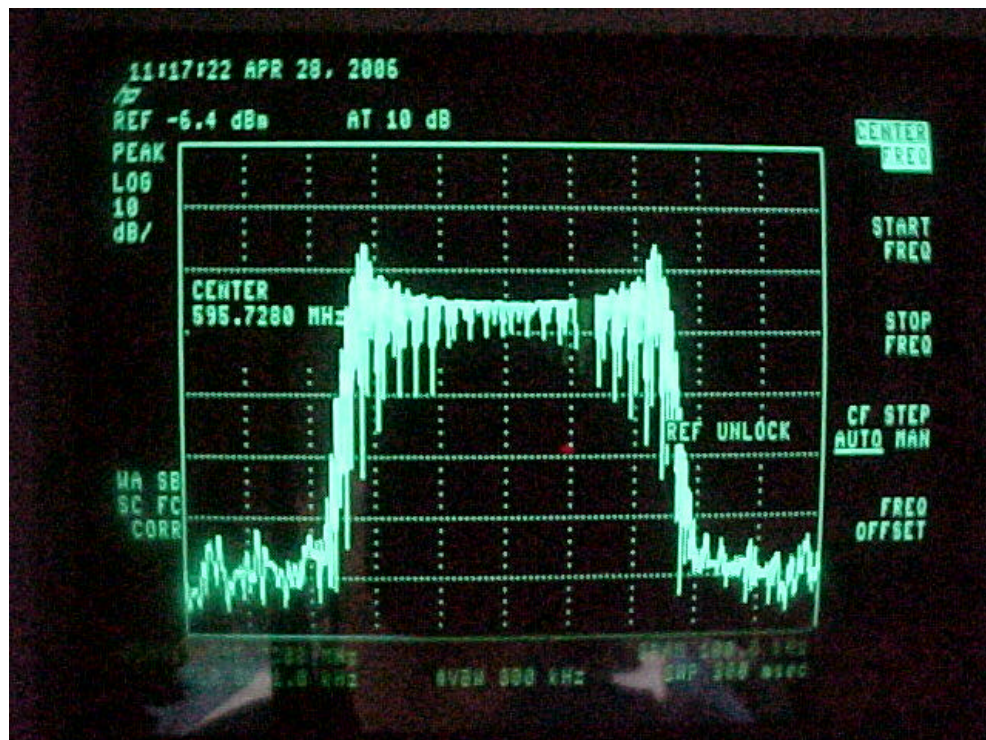
Figure 4-7. Channel-Occupied Bandwidth
