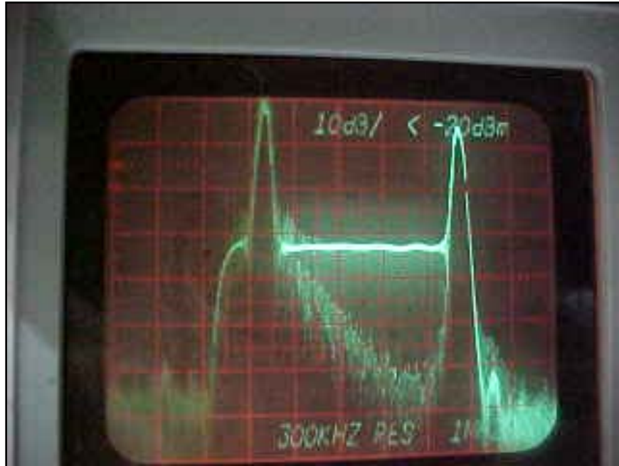
Figure 4-7. Channel Occupied Bandwidth
