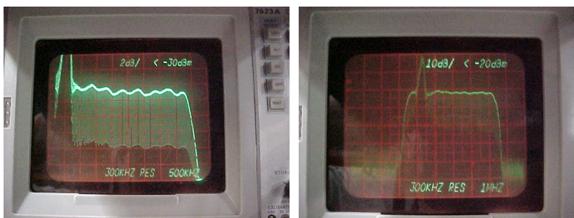
Figure 4-4. Spectrum Analyzer Results
