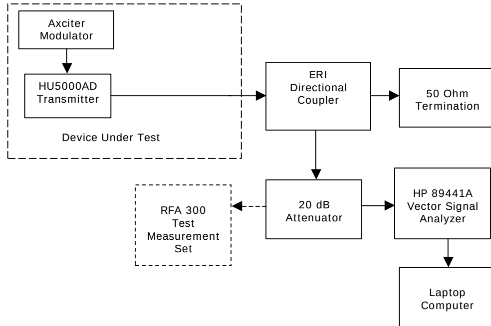
Figure 4-2. Typical Demodulation Test Setup
