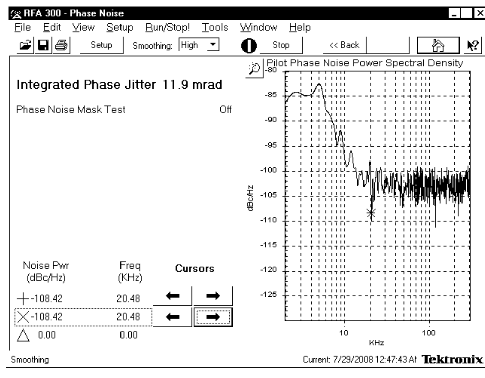
Figure 4-6. Phase Noise Plot
