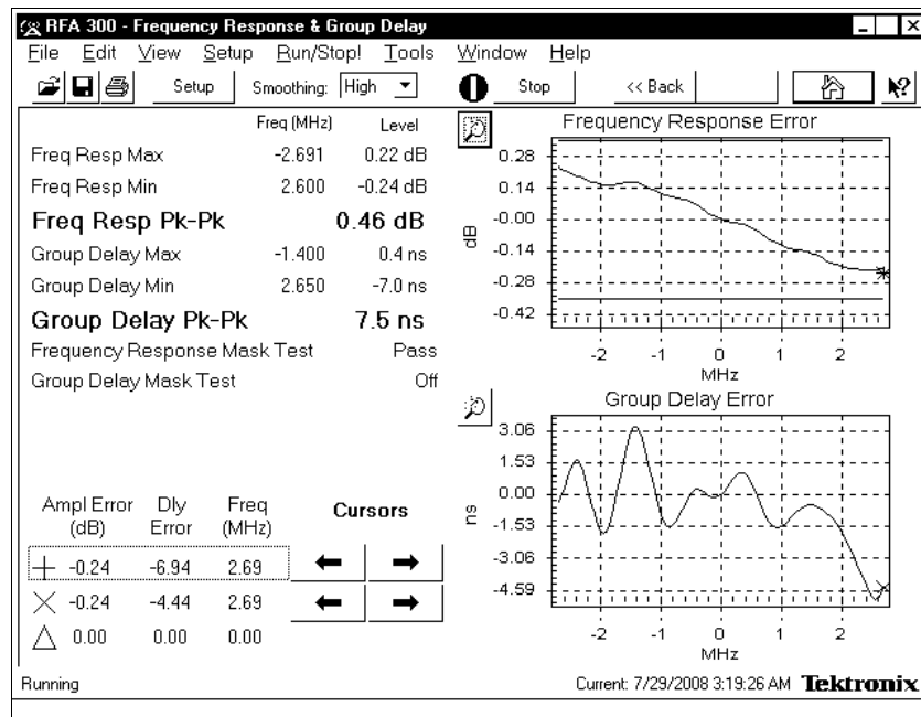
Figure 4-4. Frequency Response and Group Delay Plots
