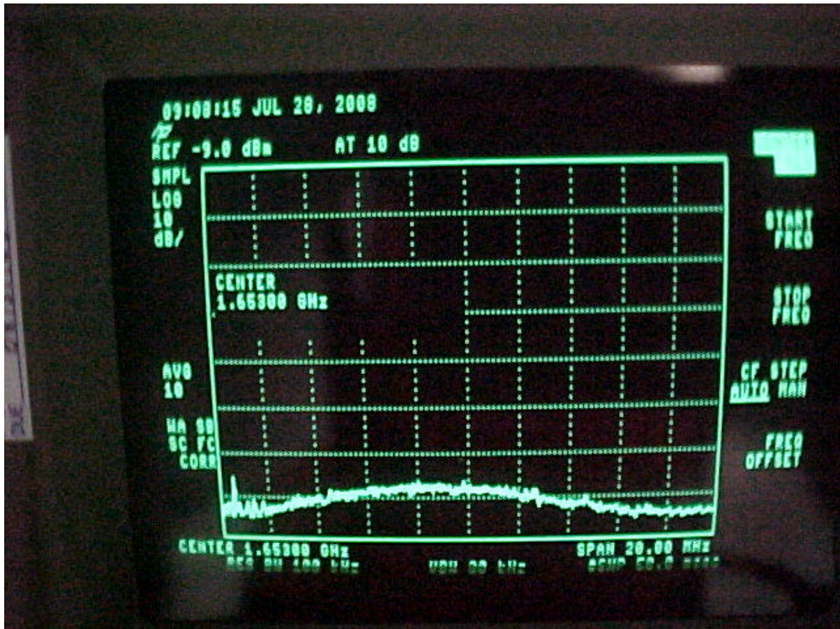
Figure 4-8C. Third Harmonic (1653 MHz) = -77 dBm (Pre-Filter)
