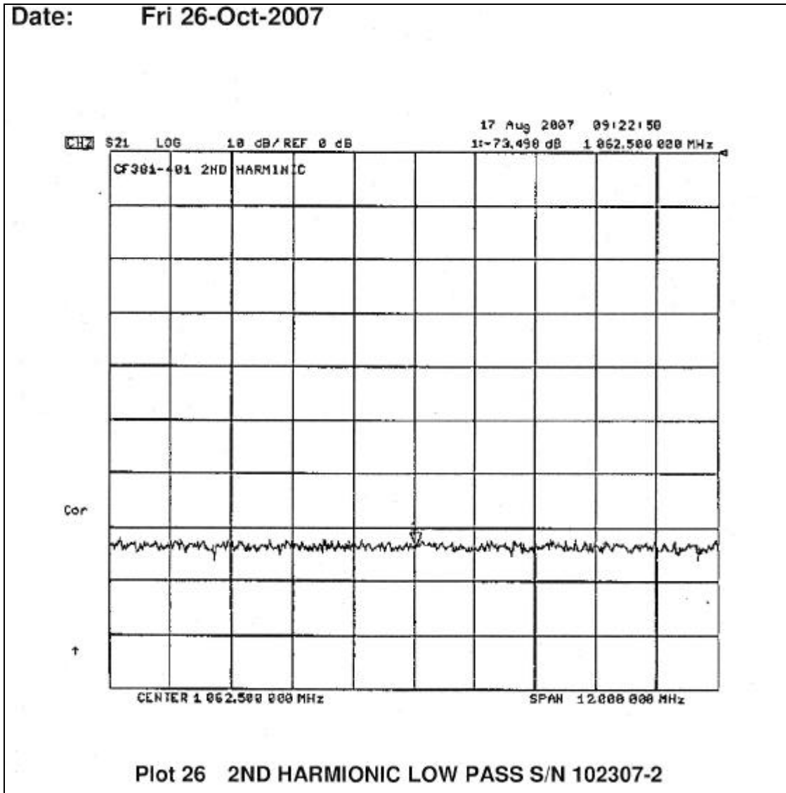
Figure 4-8E. 2 nd Harmonic (Typical Performance)
