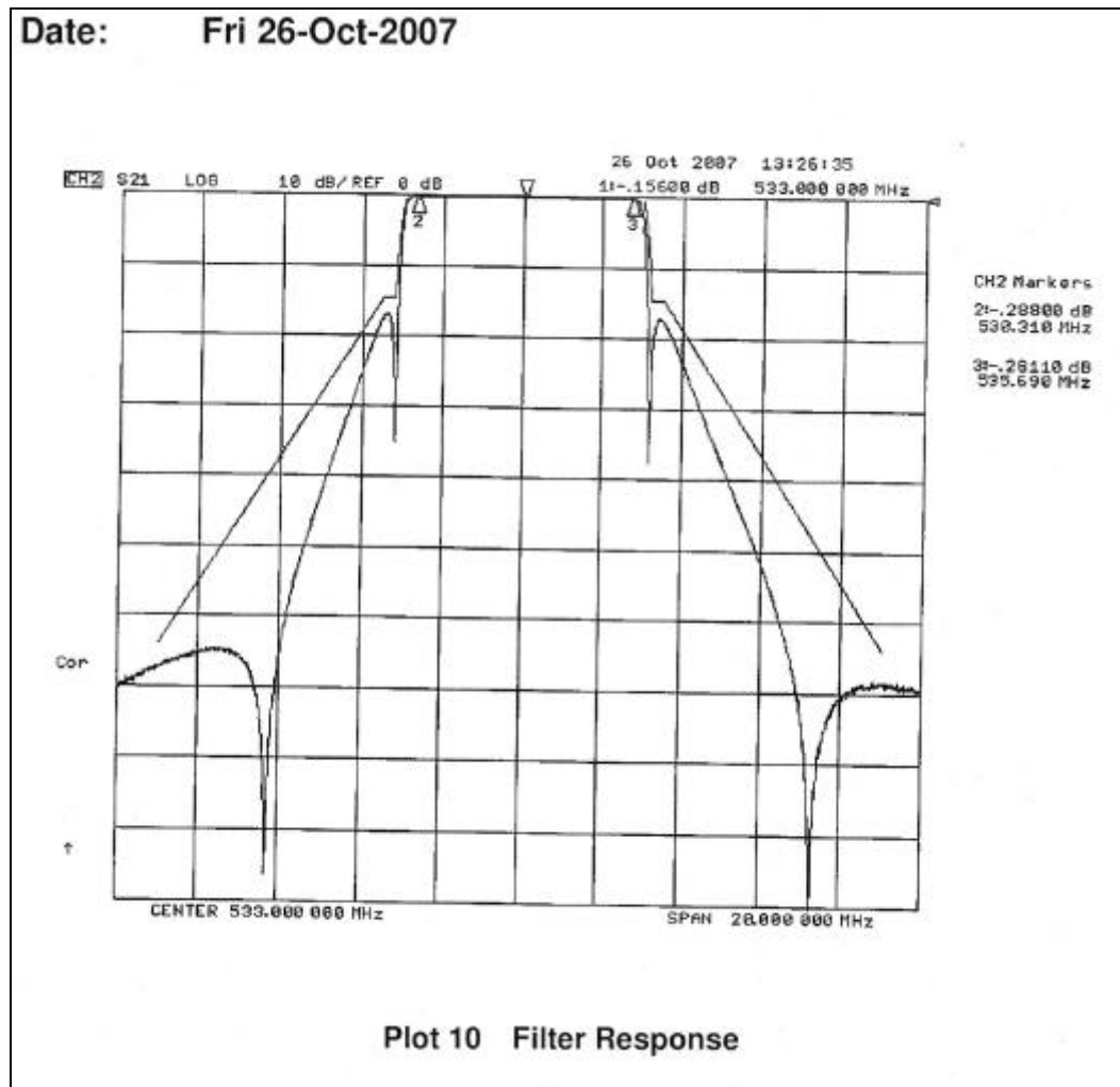
Figure 4-8D. Filter Response (Typical Performance)
