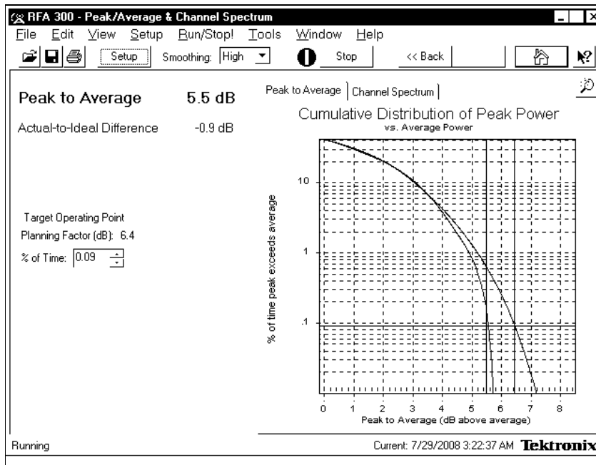
Figure 4-5. Peak to Average Plot
