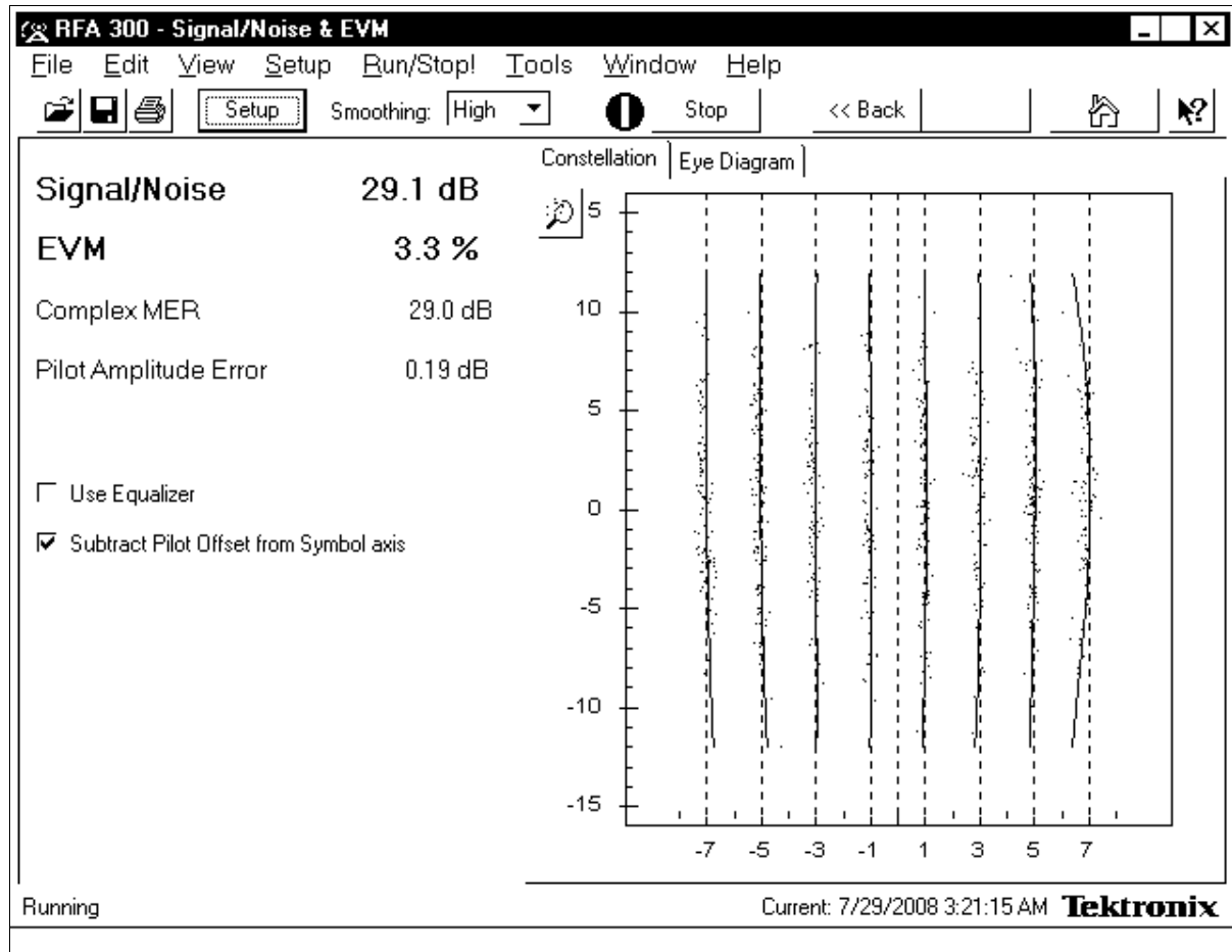
Figure 4-3. EVM and SNR Measurement
