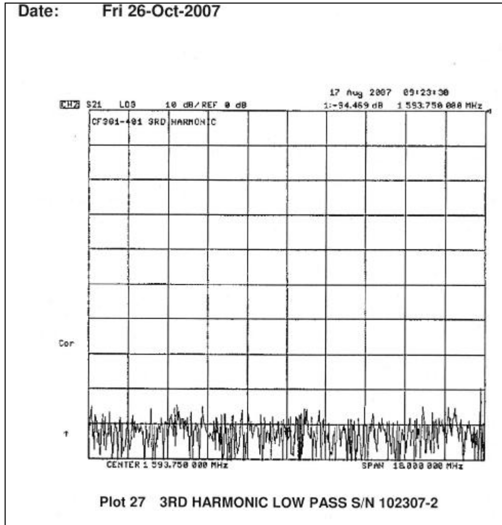
Figure 4-8F. 3rd Harmonic (Typical Performance)
