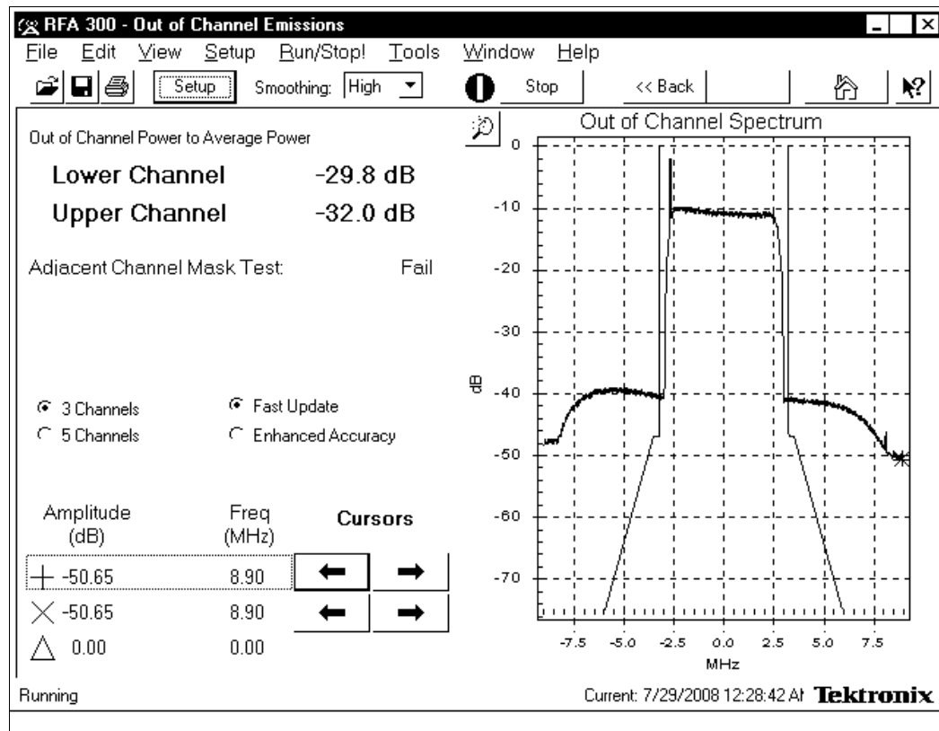
Figure 4-8H. Out of Band Emissions Plot (Pre-Filter)
