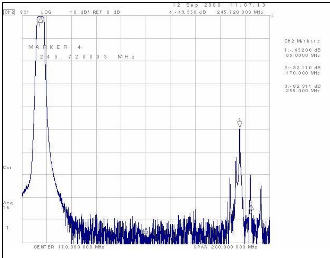
Figure 4-8F. Harmonics Plot (Post Filter)
