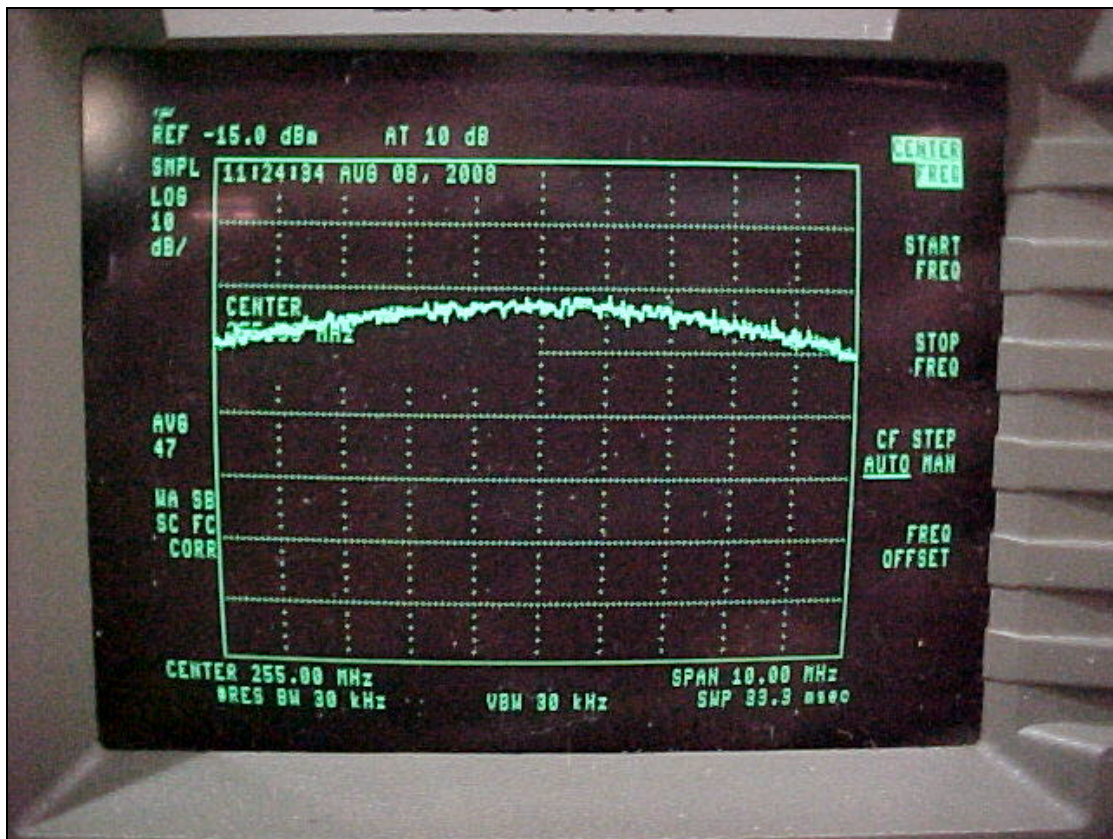
Figure 4-8C. Third Harmonic (255.00 MHz) = -37.0 dBm (Pre-Filter)
