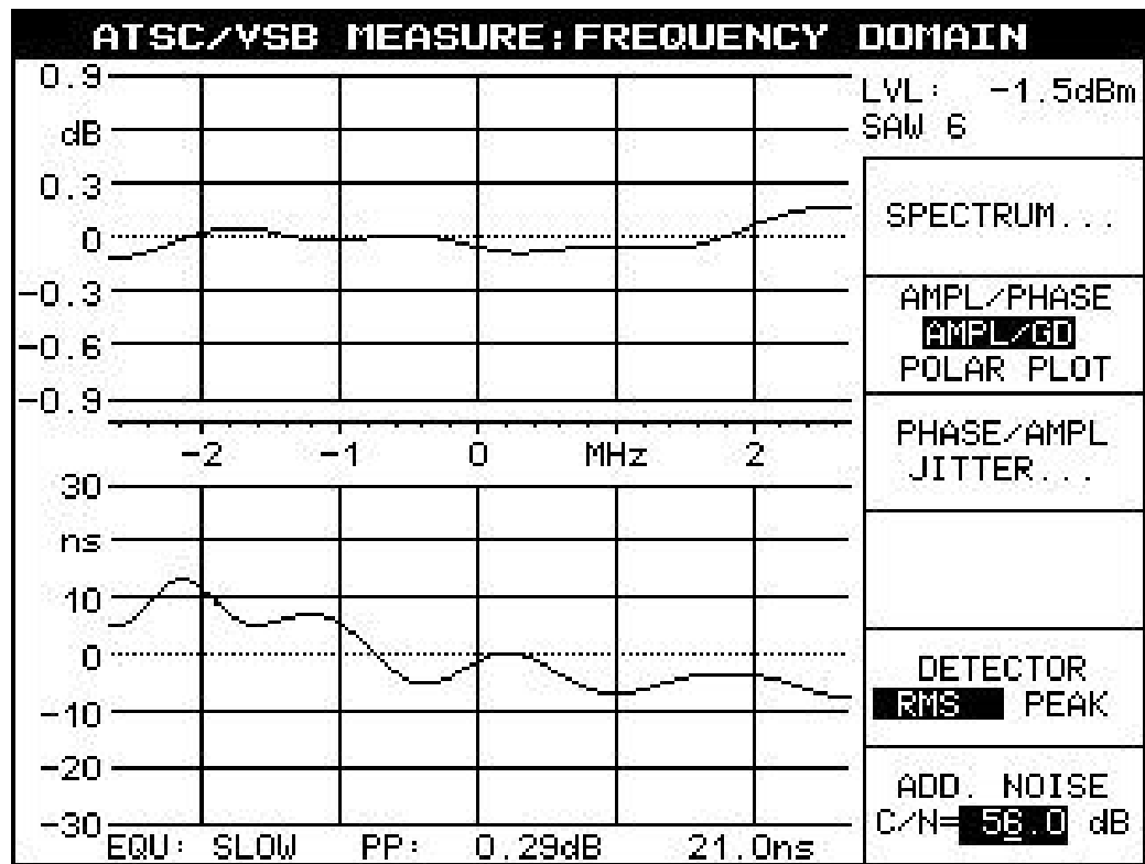
Figure 4-4. Frequency Response and Group Delay Plots
