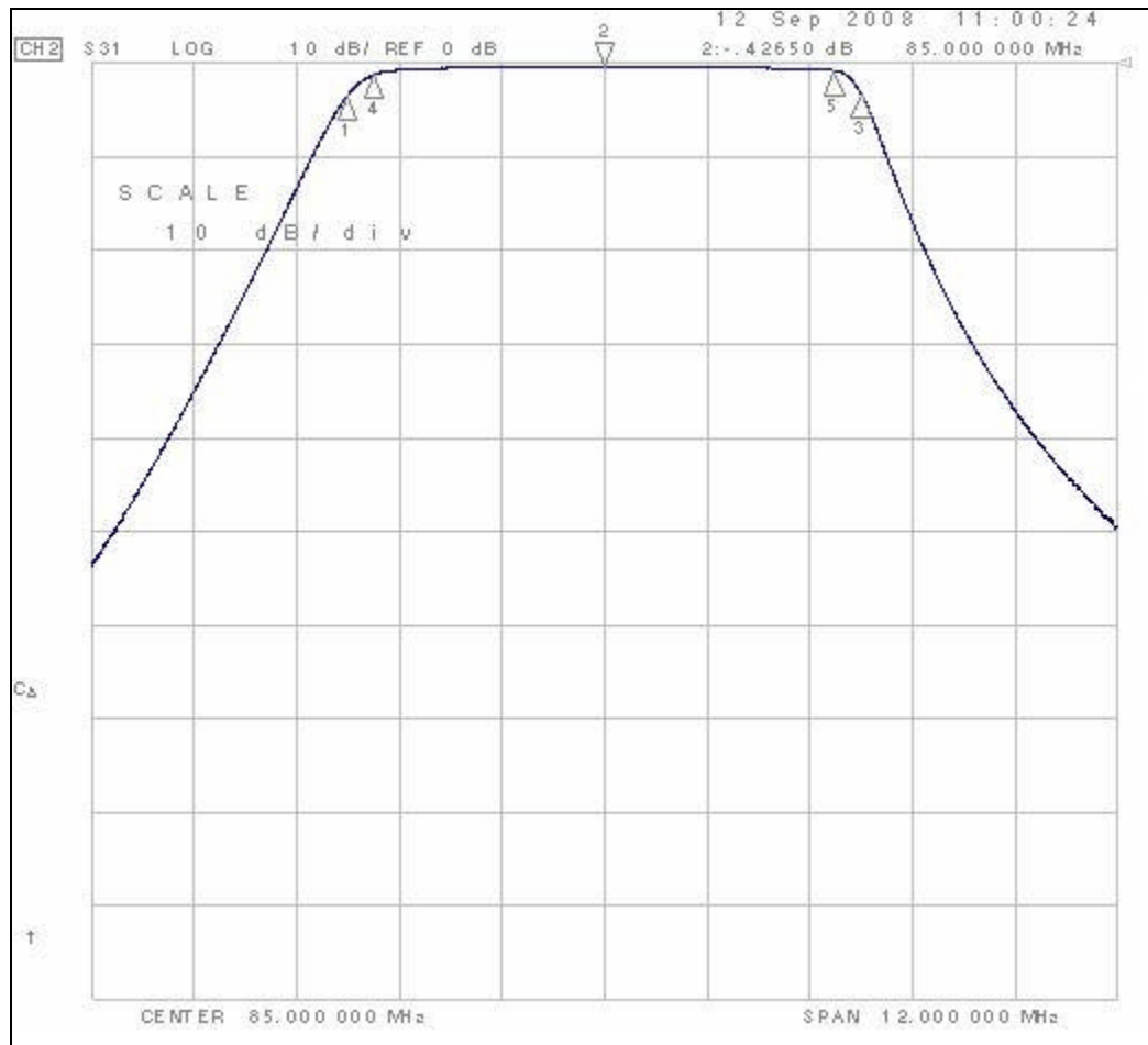
Figure 4-8D. Filter Response
