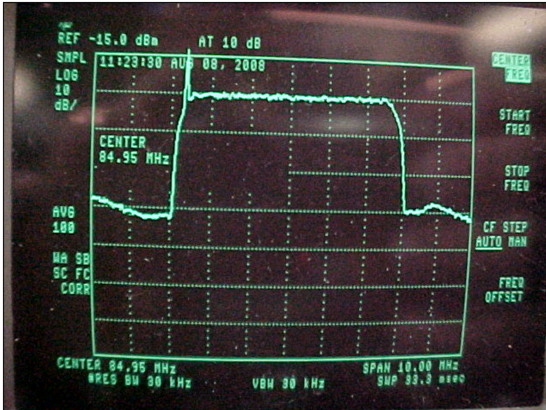
Figure 4-8A. Reference (85.00 MHz) = -25.0 dBm (Pre-Filter)
