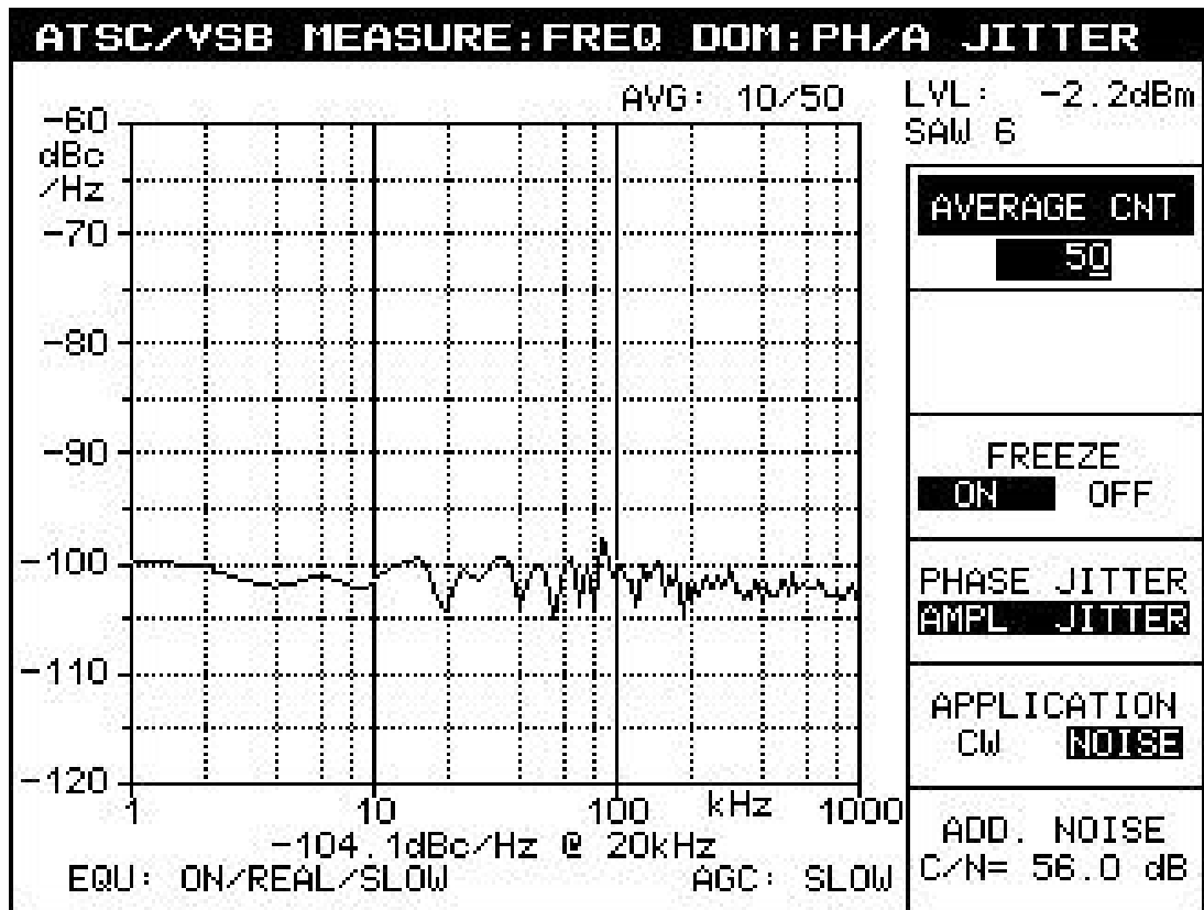
Figure 4-6. Phase Noise Plot
