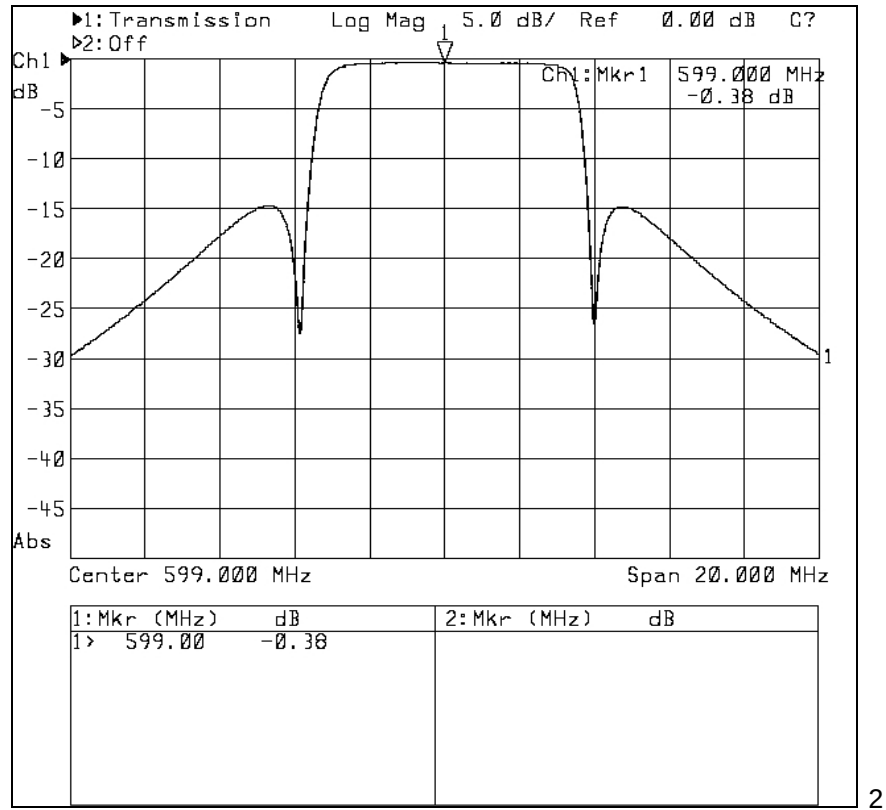
Figure 4-8B. Simple Mask Filter Response
