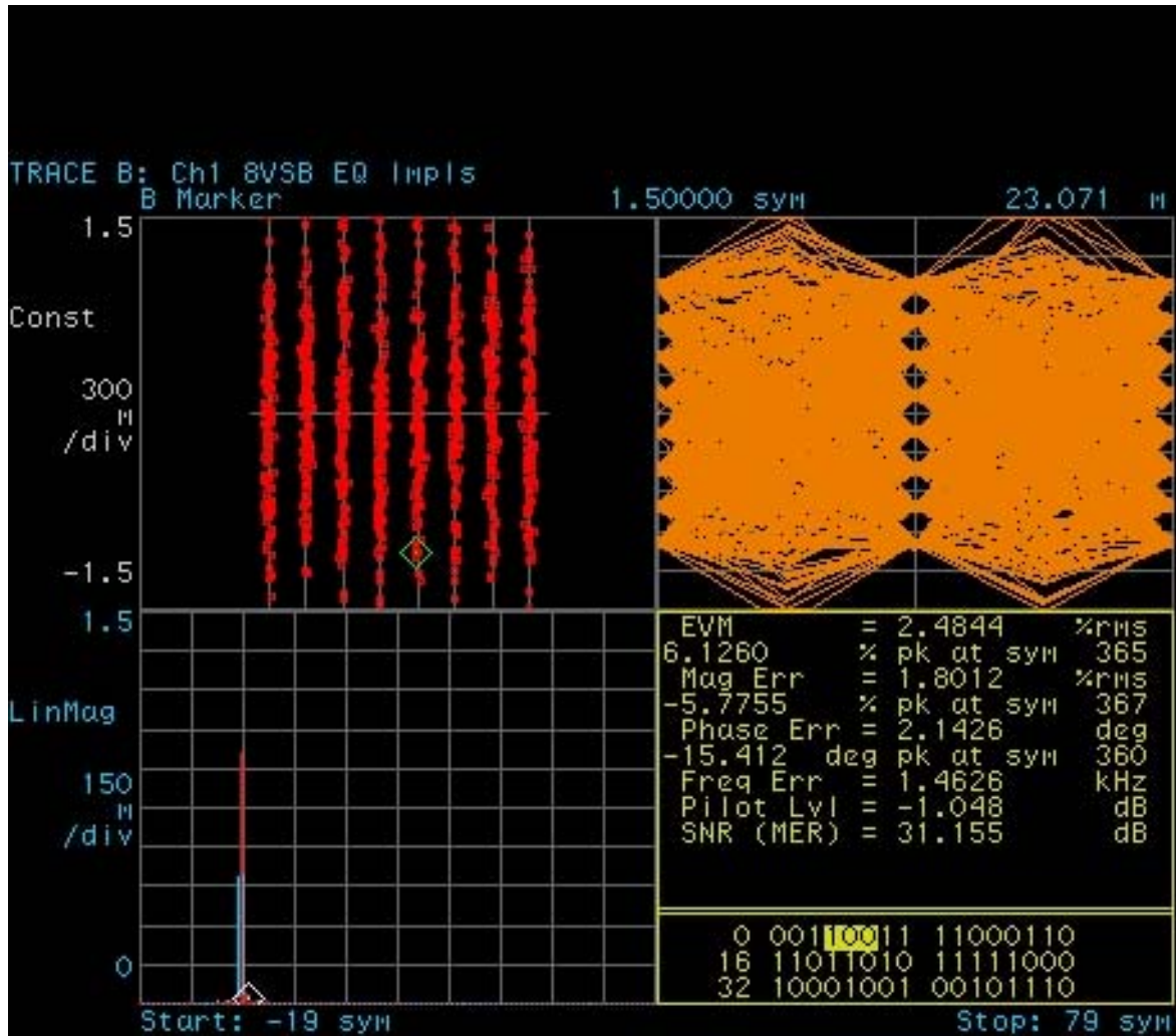
Figure 4-3. Constellation Diagram
