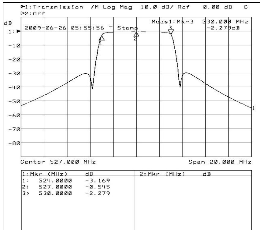
Figure 4-8D. Bandpass Filter response
