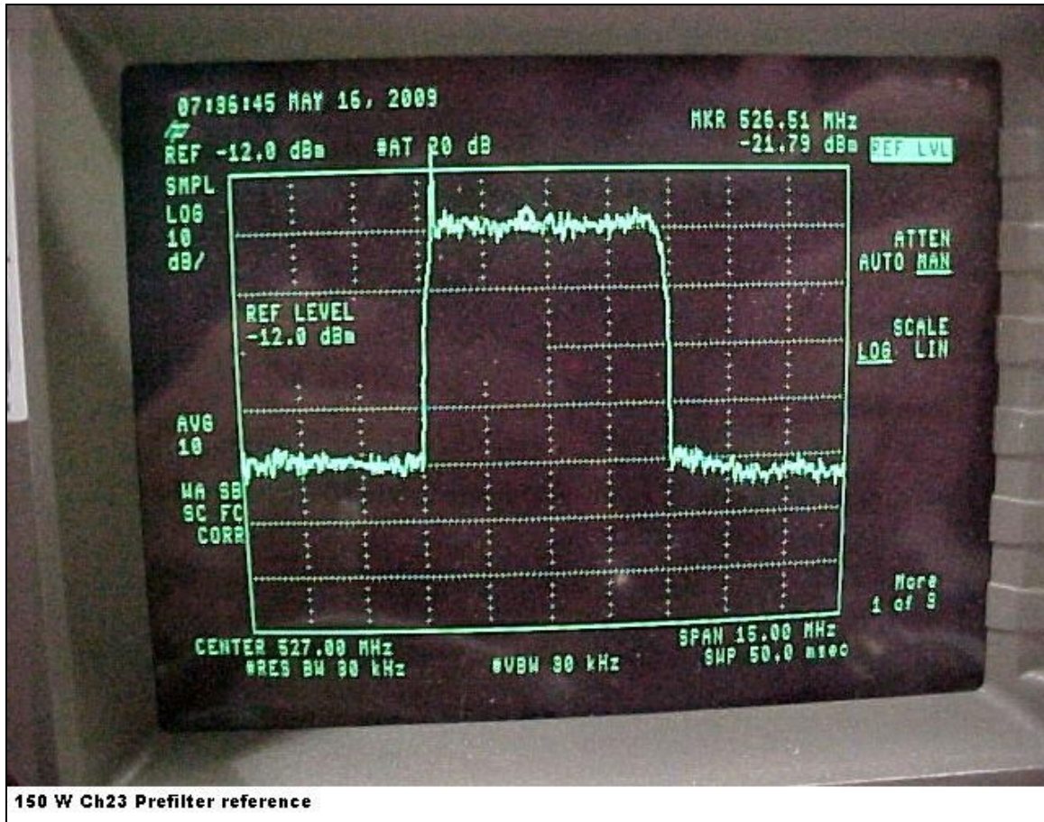
Figure 4-8A. Reference (527.00 MHz) = 0dBc (Pre-Filter)
