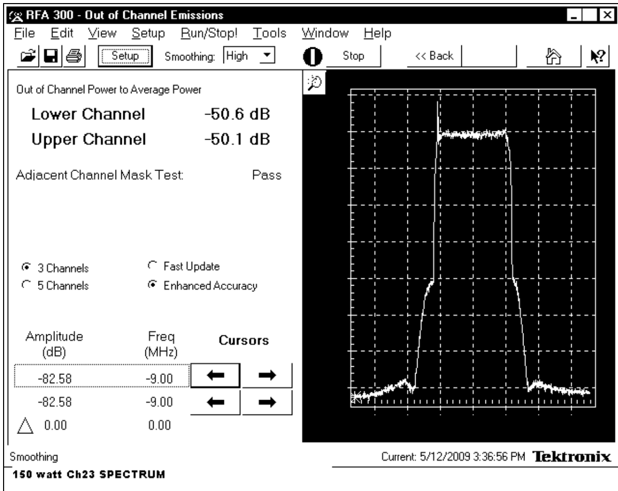
Figure 4-8J. Out of Band Emissions (Post Filter)
