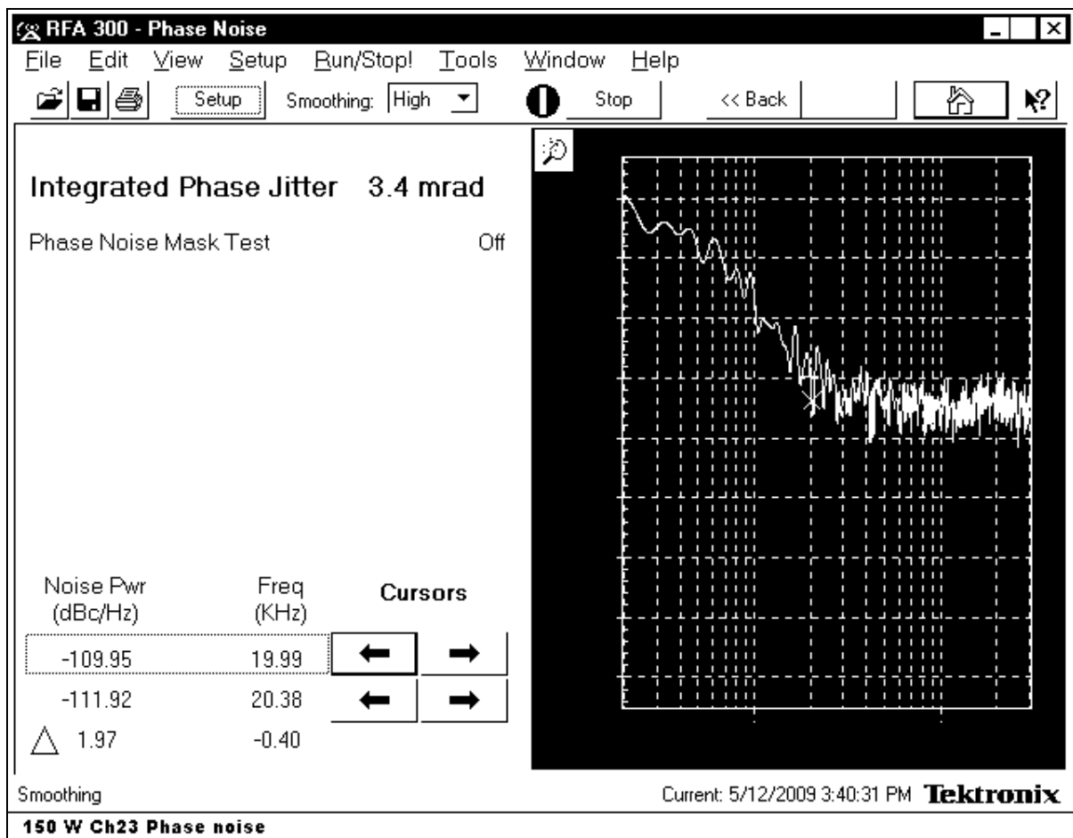
Figure 4-6. Phase Noise Plot
