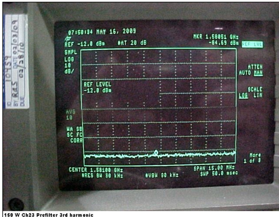
Figure 4-8C. Third Harmonic (1581.00 MHz) = -62 dBc (Pre-Filter)
