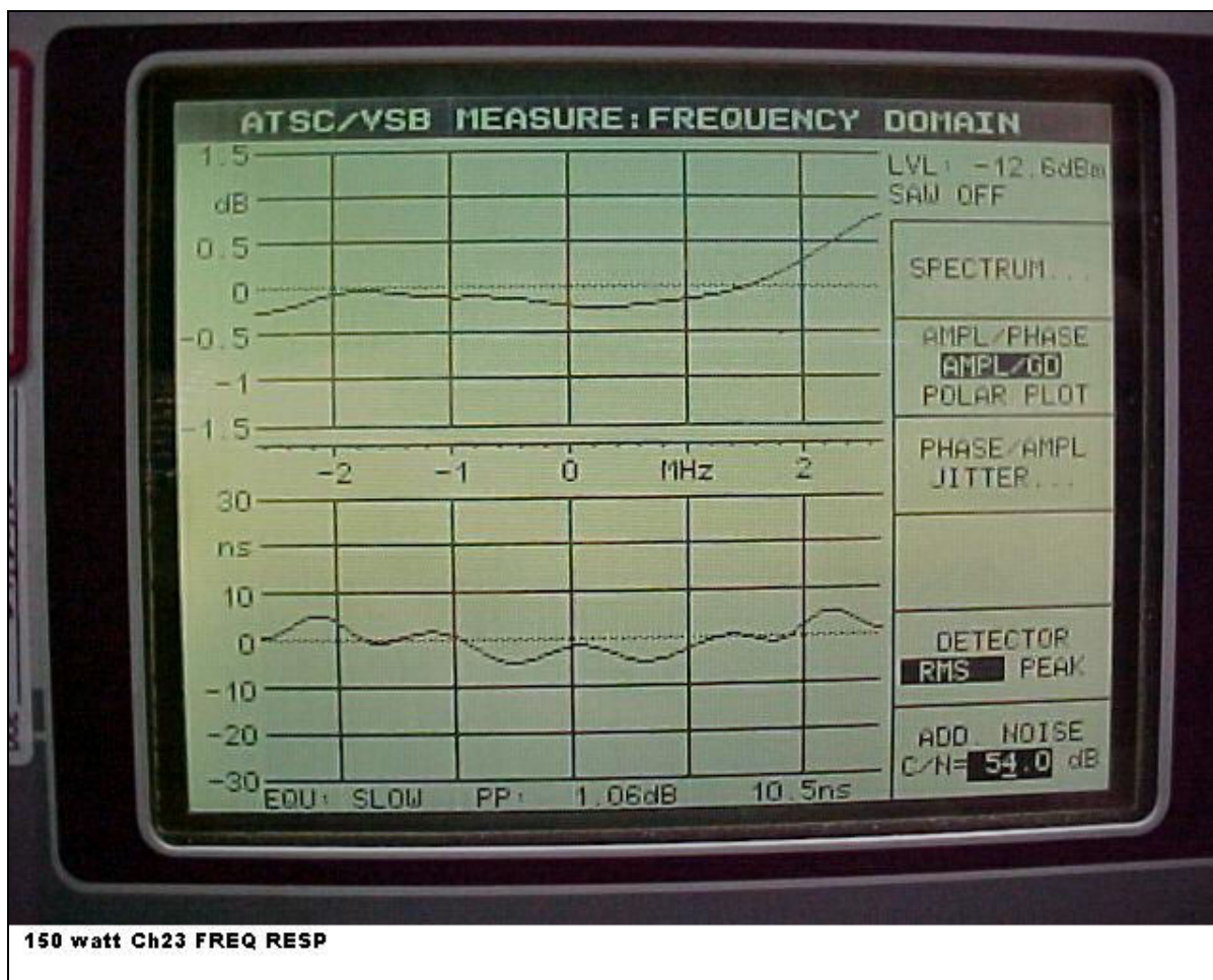
Figure 4-4. Frequency Response Plot
