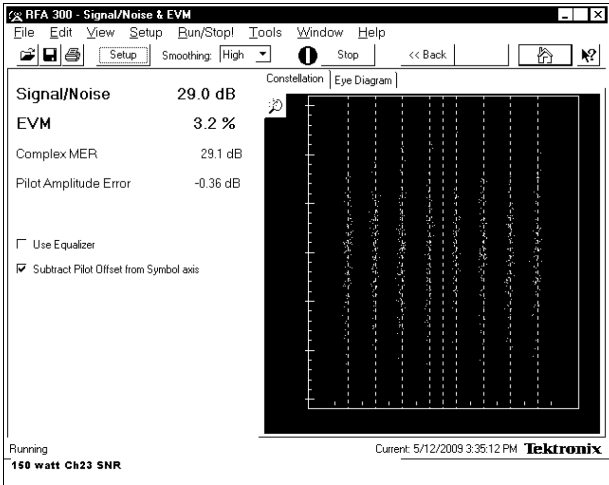
Figure 4-3. Constellation Diagram
