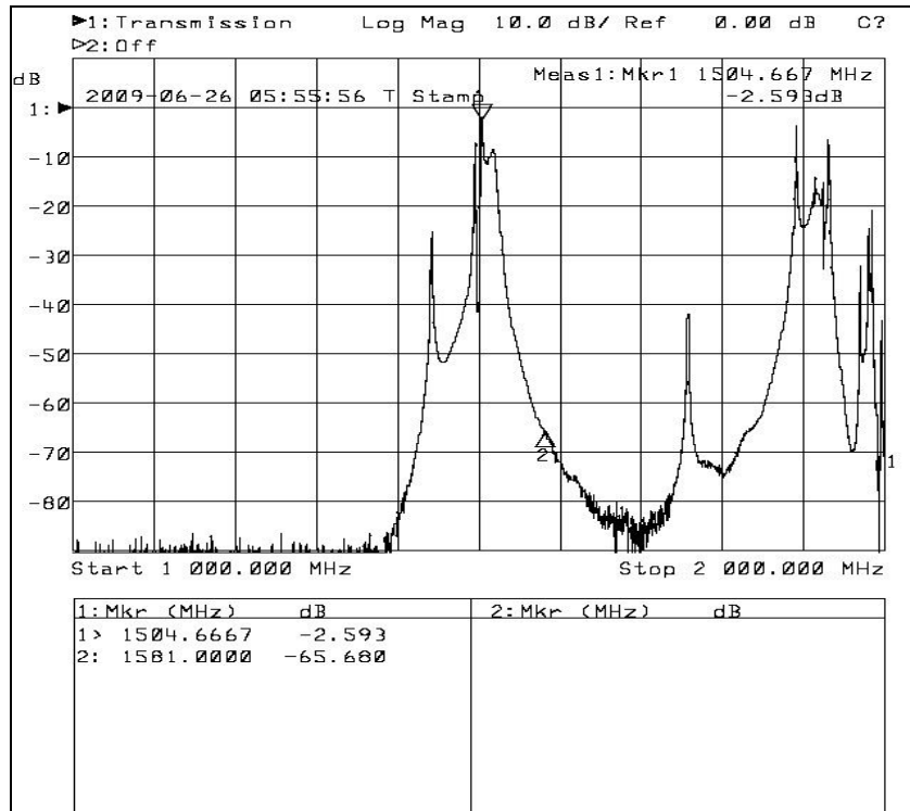
Figure 4-8F. Bandpass Filter response
