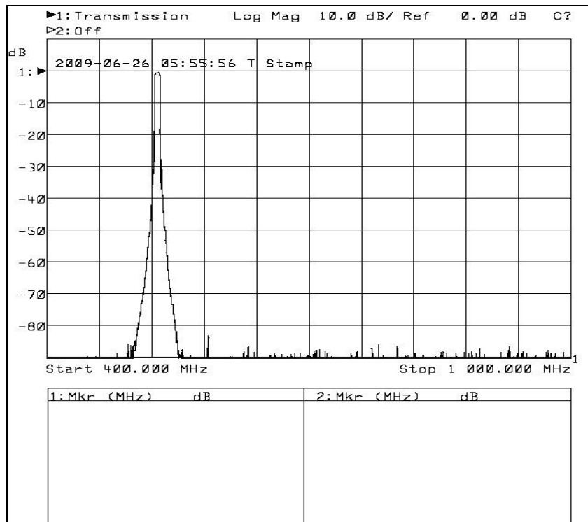
Figure 4-8E. Bandpass Filter response
