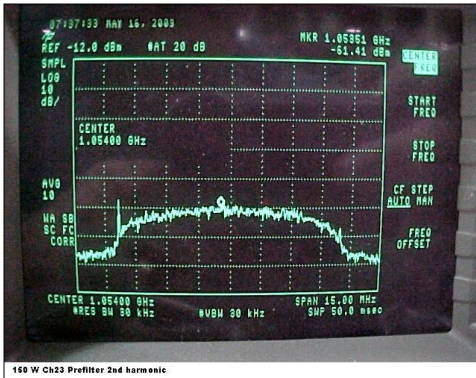
Figure 4-8B. Second Harmonic (1054.00 MHz) = -50 dBc(Pre-Filter)
