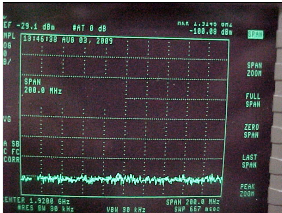
Figure 4-8C. Third Harmonic (1923.00 MHz) = -60 dBc (Pre-Filter)
