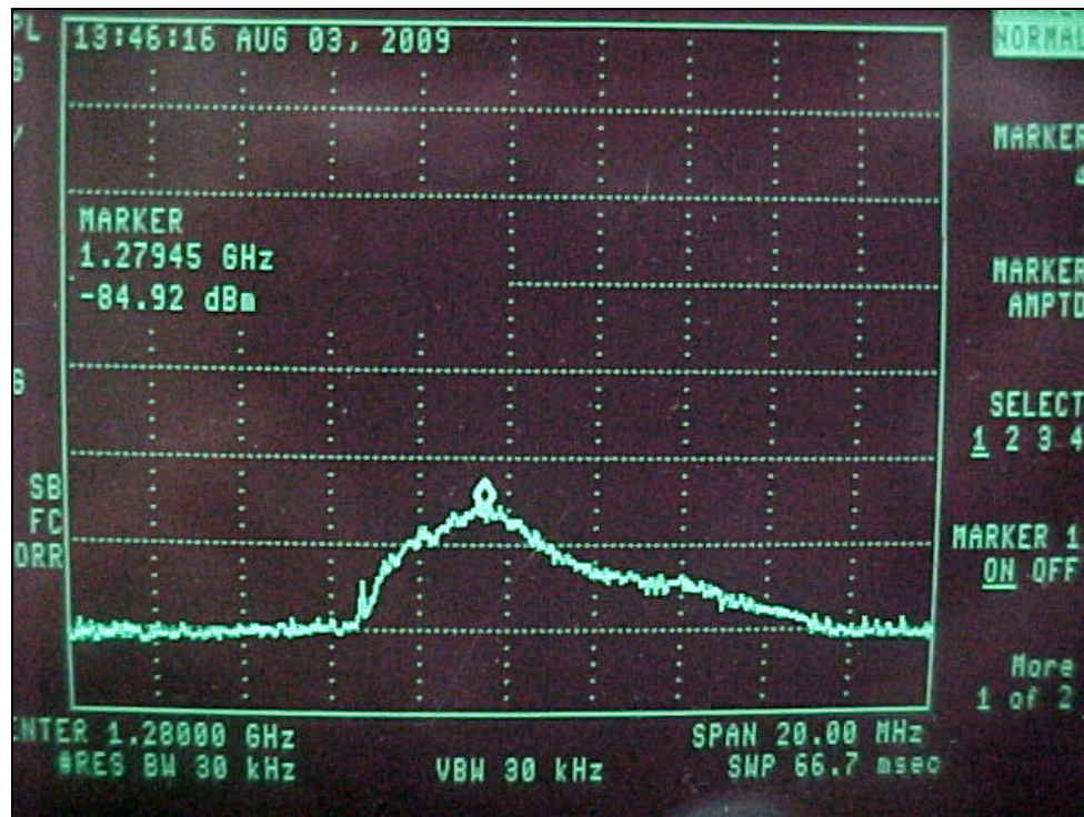
Figure 4-8B. Second Harmonic (1282.00 MHz) = -46 dBc (Pre-Filter)
