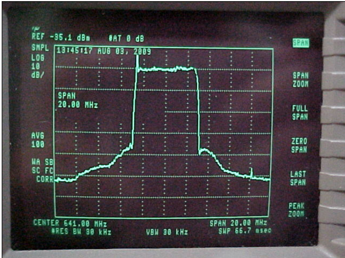
Figure 4-8A. Reference (641.00 MHz) = 0dBc (Pre-Filter)
