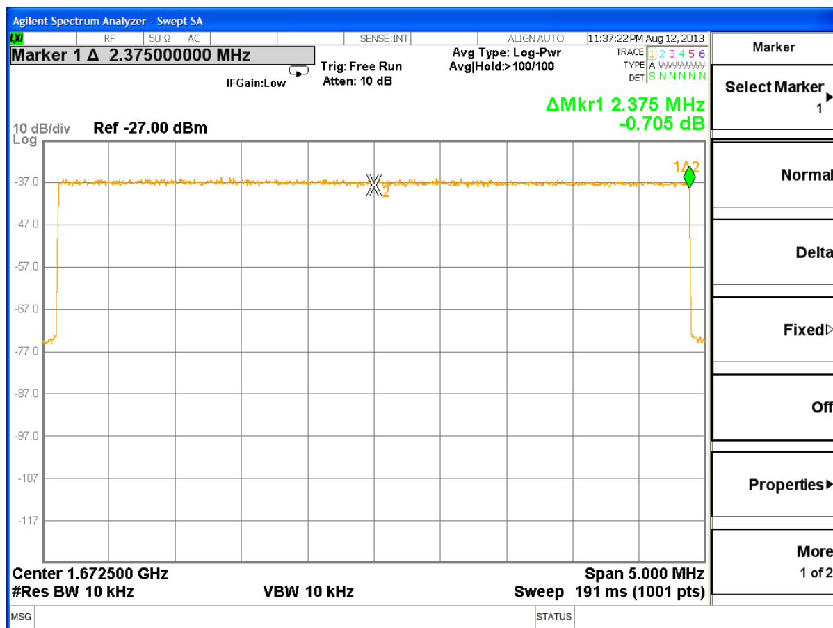
Figure 4-6. Channel Occupied Bandwidth (upper channel edge)
