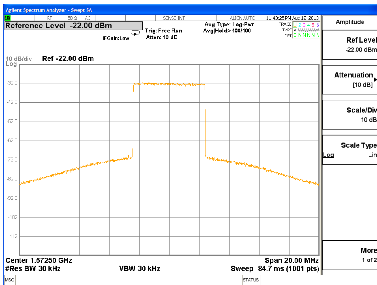
Figure 4-8. Conducted Spurious Emissions (before channel filter)
