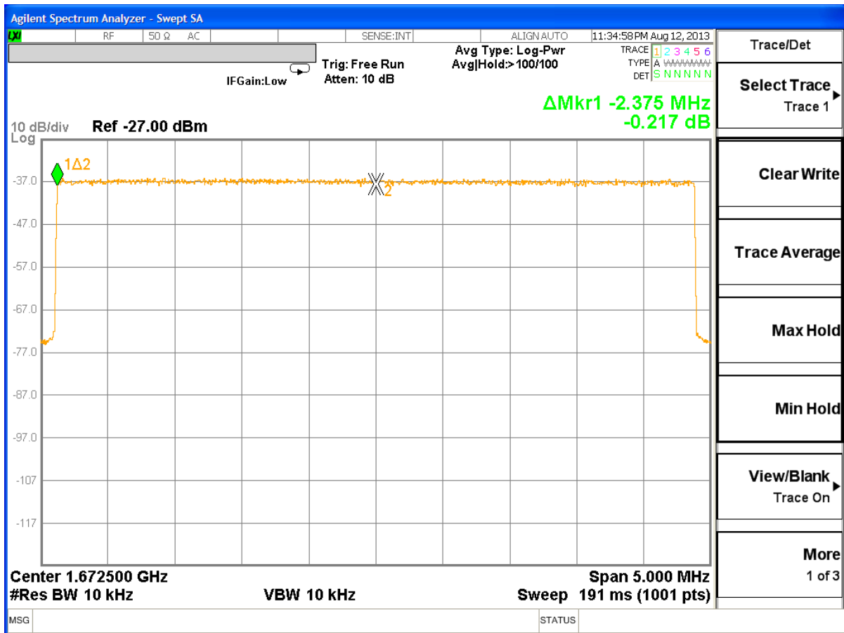
Figure 4-5. Channel Occupied Bandwidth (lower channel edge)
