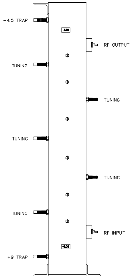
Figure 7-2. Bandpass Filter
