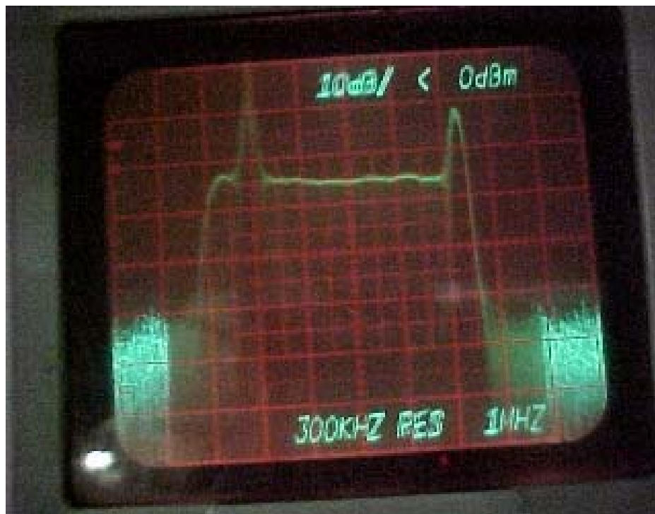
Figure 4-7. Channel-Occupied Bandwidth
