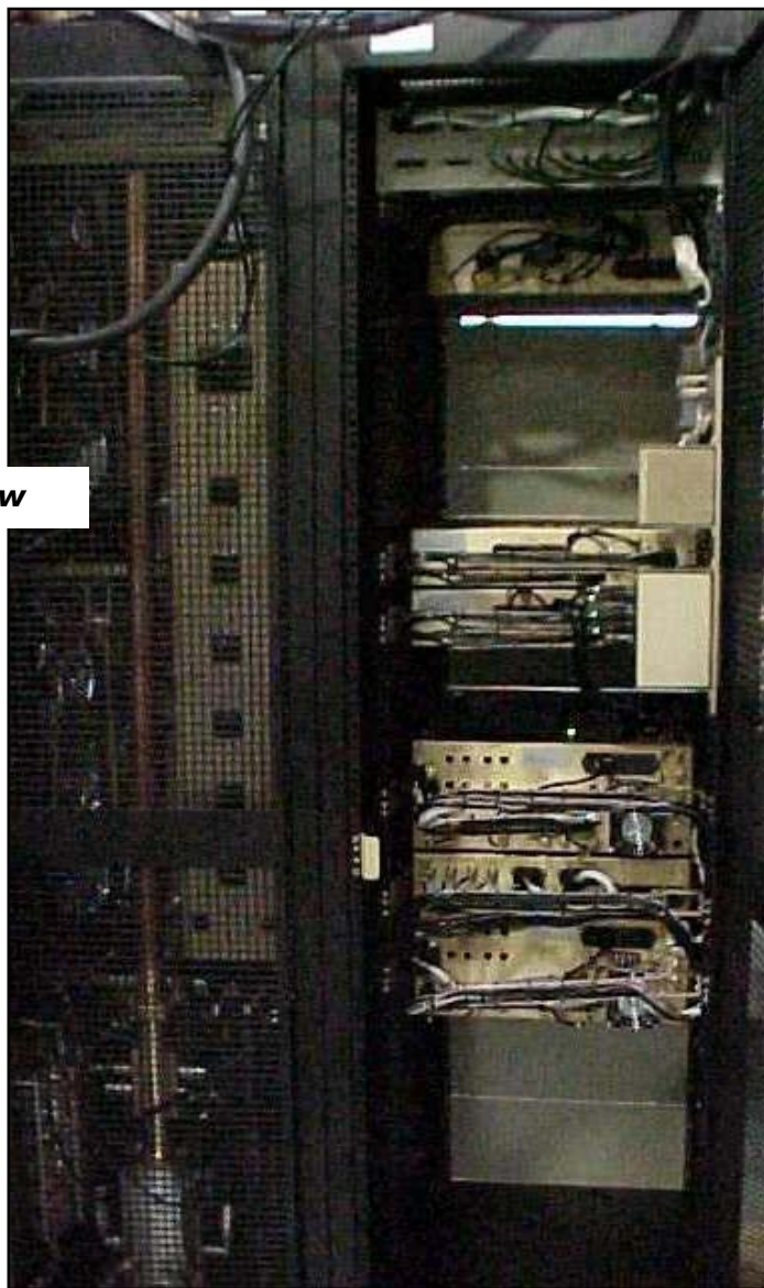
Exciter Cabinet
