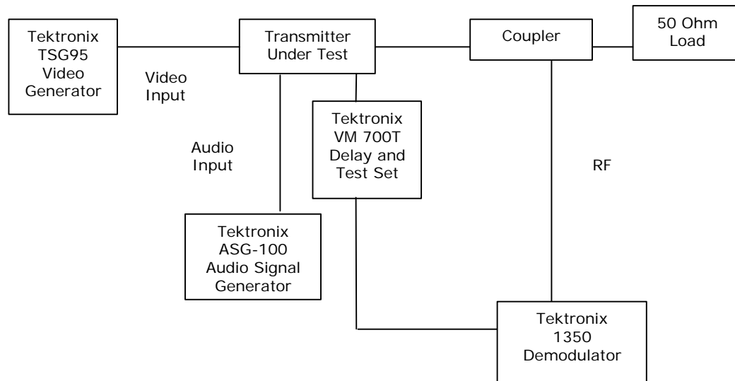
Figure 4-5. Test Setup for Measuring FM Deviation and Distortion
