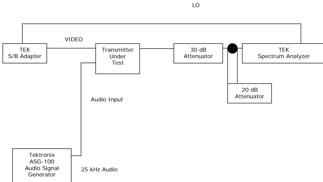
Figure 4-6. Test Setup for Occupied Bandwidth Spectrum Analysis
