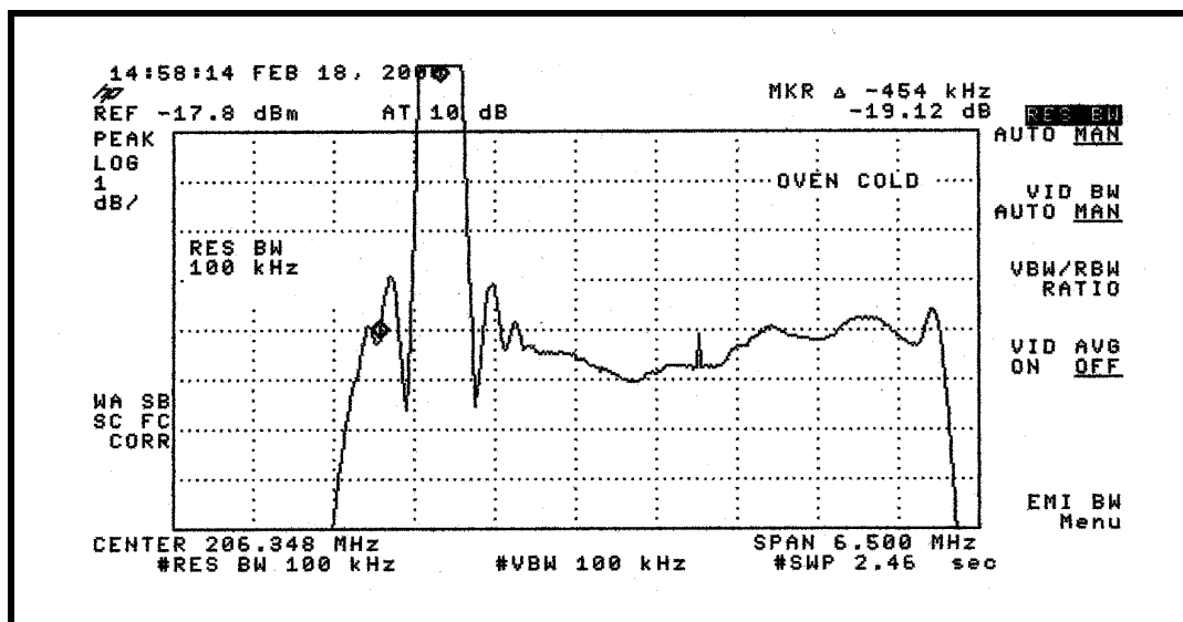
Figure 4-3. Graph of Detected Video Frequency Response
