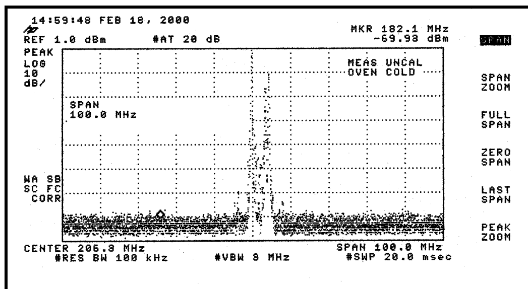
Figure 4-9. Products Above the 70-dB Noise Floor of the Spectrum Analyzer (1 of 2)
