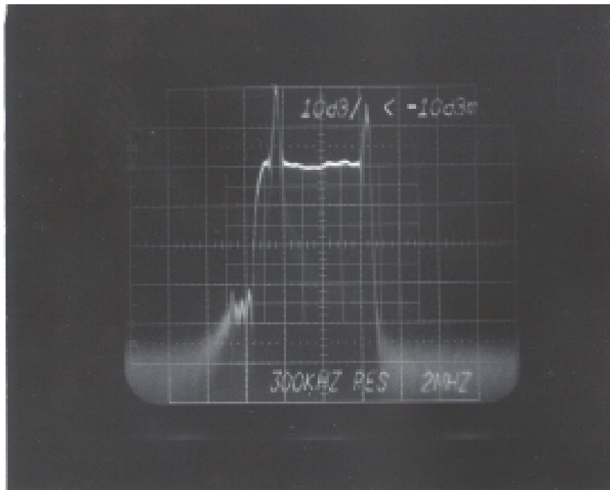
Figure 4-7. Channel-Occupied Bandwidth
