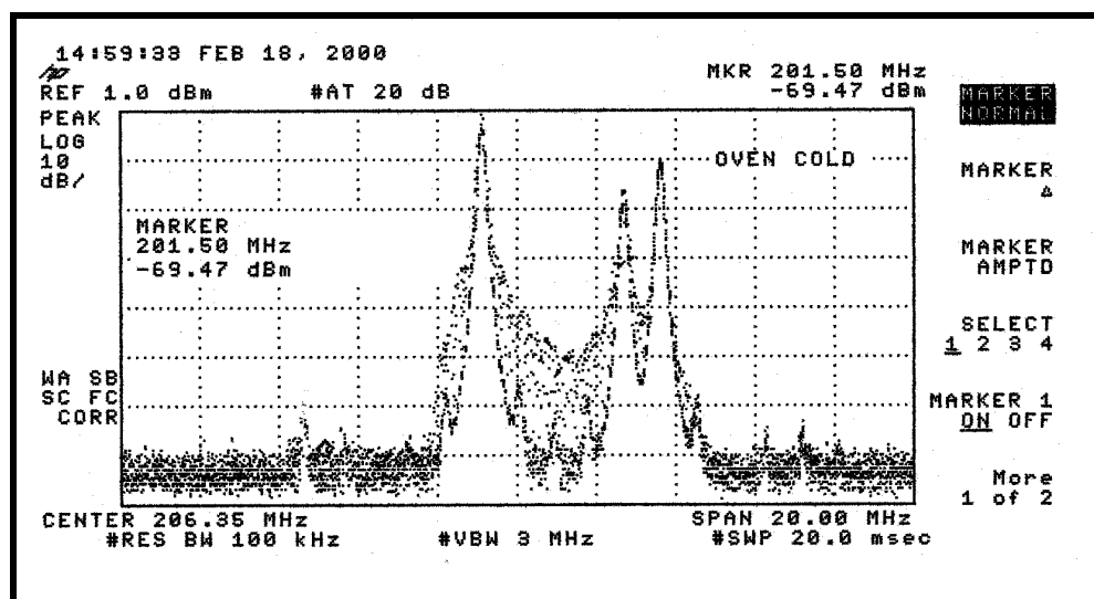
Figure 4-10. Products Above the 70-dB Noise Floor of the Spectrum Analyzer (2 of 2)
