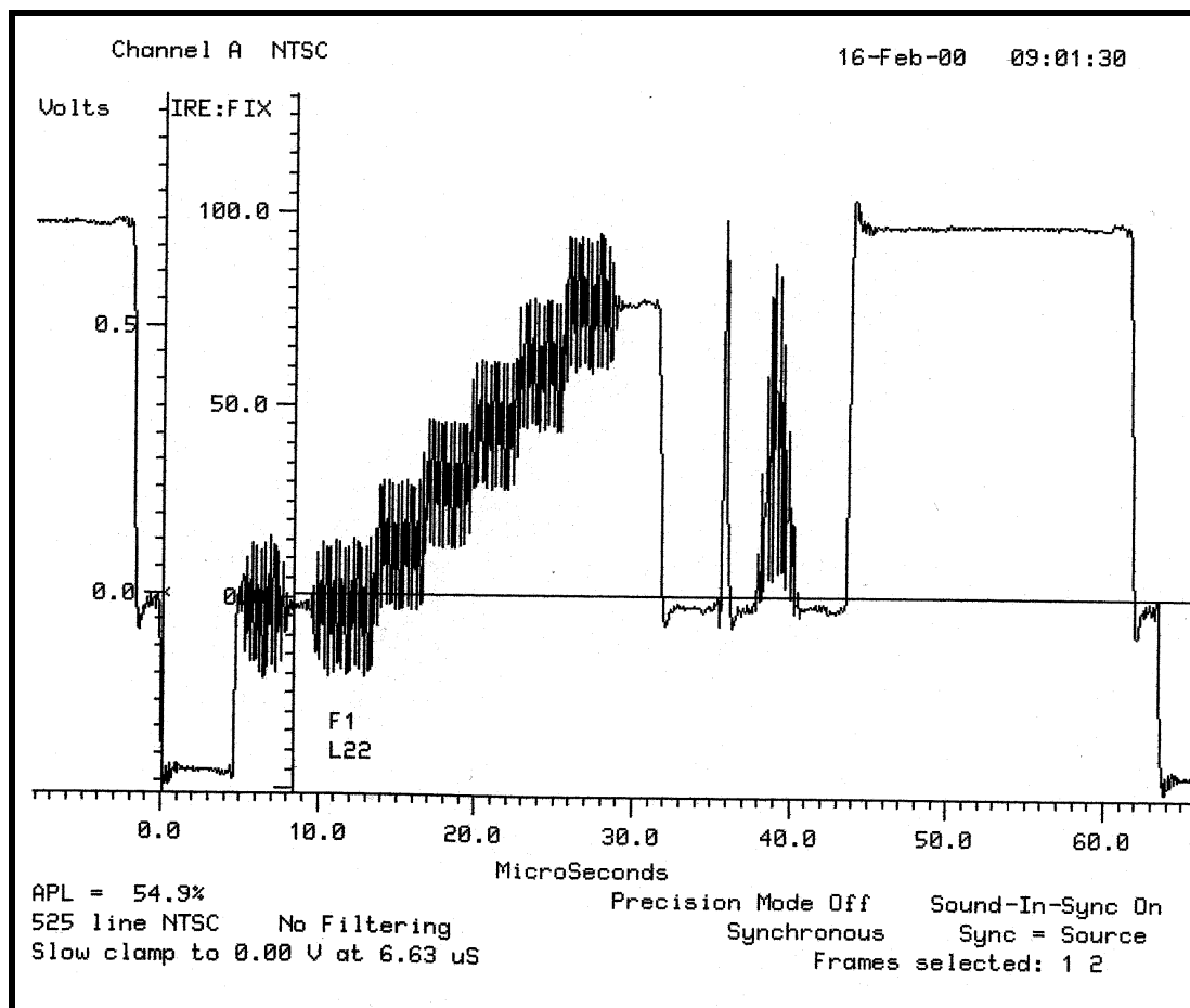
Figure 4-2. Substantially Linear Transfer Characteristics of the Transmitter as a Demodulated Video Waveform
