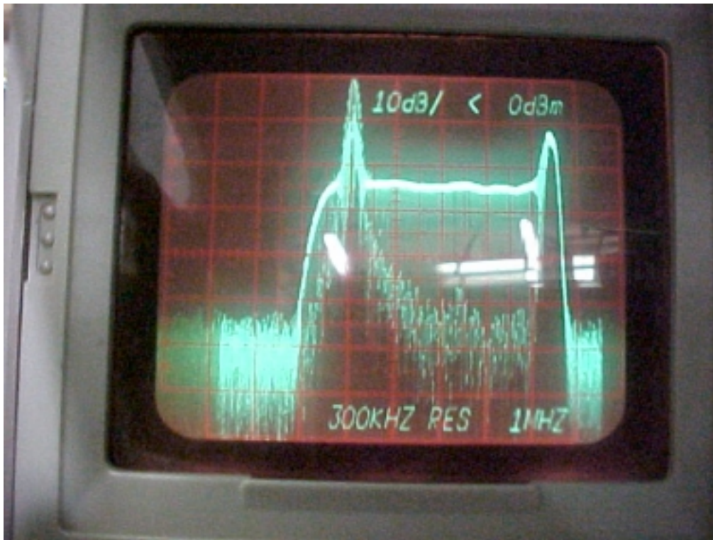
Figure 4-7. Channel-Occupied Bandwidth
