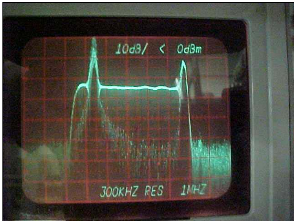
Figure 4-7. Channel-Occupied Bandwidth
