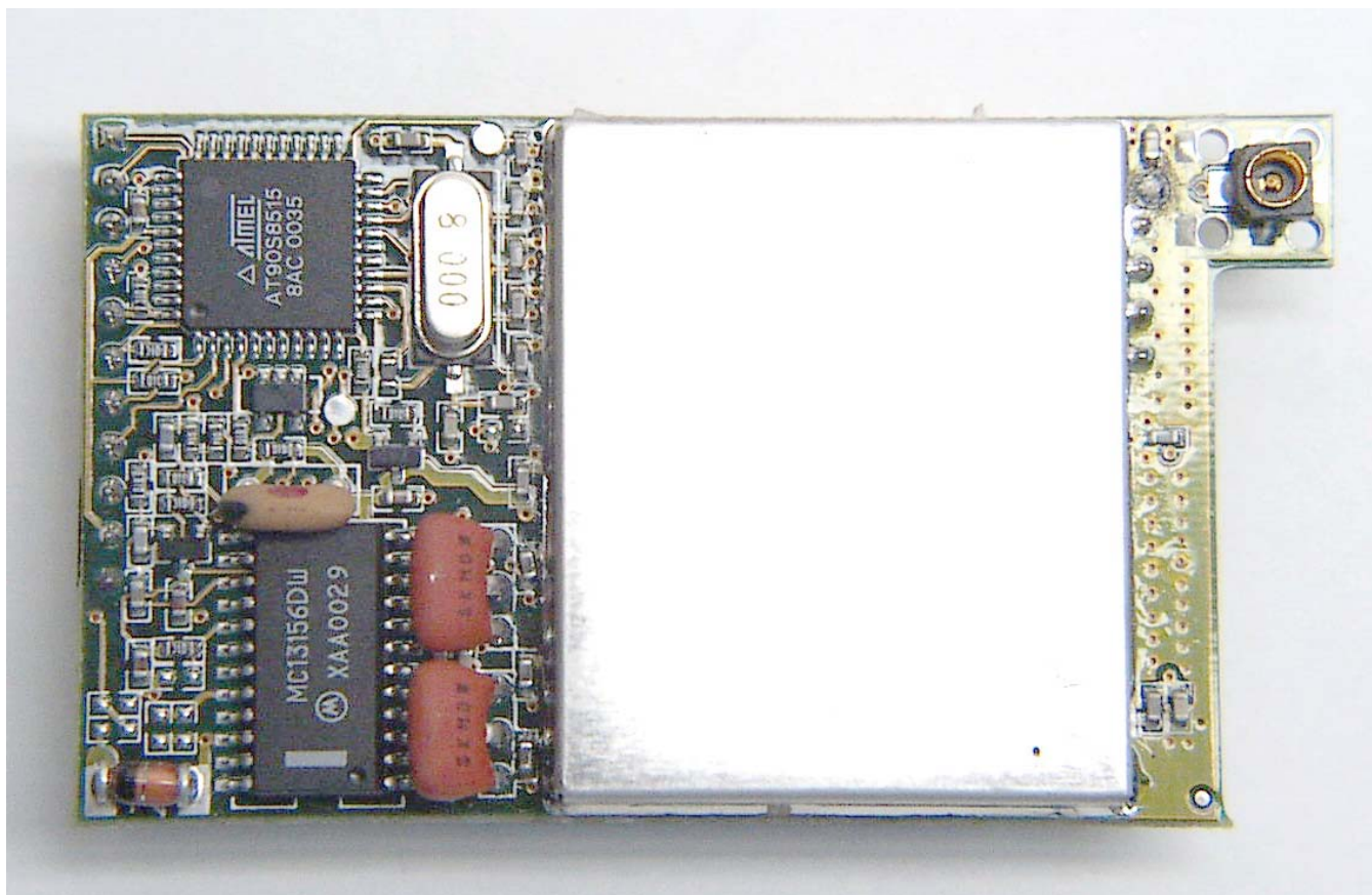
9XSTREAM with RF Can Installed (Top View)
